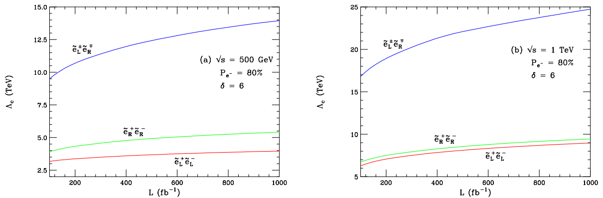
FIG. 3: 95% C.L. search reach for \Lambda_c in each production channel as a function of integrated luminosity for \sqrt{s} = 0.5 and 1.0 TeV.
