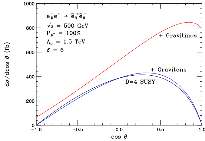
FIG. 2: The angular distribution for e_R^- e^+ \rightarrow \tilde{e}_R^+ \tilde{e}_R^- from the D = 4 supersymmetric model I, plus the addition of bulk graviton KK tower exchange, and with bulk gravitino KK tower exchange, corresponding to the bottom, middle, and top curves, respectively.
