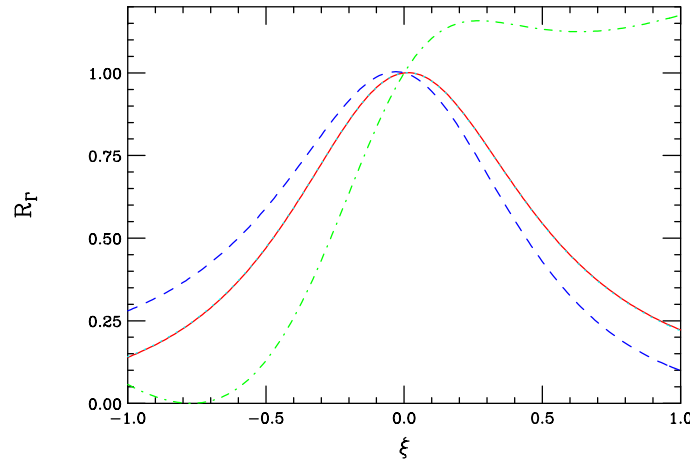
FIG. 7: The effect of mixing on the partial widths of a 125 GeV Higgs boson, described by the parameter \xi , assuming v/\Lambda = 0.2 and a radion mass of 300 GeV as discussed in the text. The solid(dash-dotted, dashed, dotted) corresponds to the ZZ/W^+W^- (gg, \gamma\gamma, \bar{f}f) final states.
