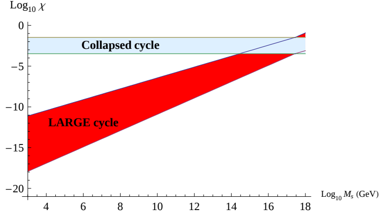
Figure 1: Kinetic mixing between the visible U(1) and a U(1) sitting on a collapsed cycle (upper, blue) or a hyperweak U(1) on a LARGE cycle (lower, red) as a function of the string scale.
