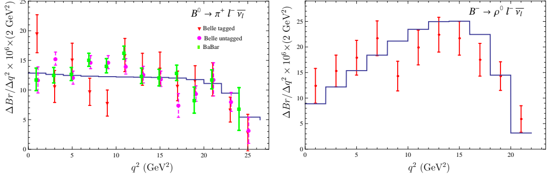
Figure 1: Comparison of predictions of our model with the recent experimental data (Belle 2011, 2013; BaBar 2012) for the B^0 \rightarrow \pi^+ l^- \nu decay and Belle (2013) data for the B \rightarrow \rho l \nu decay.
