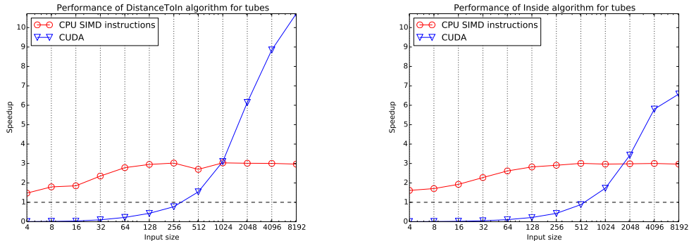
(a) Distance algorithm, 50 floating point operations per kernel execution. (b) Inside algorithm, 10 floating point operations per kernel execution.
