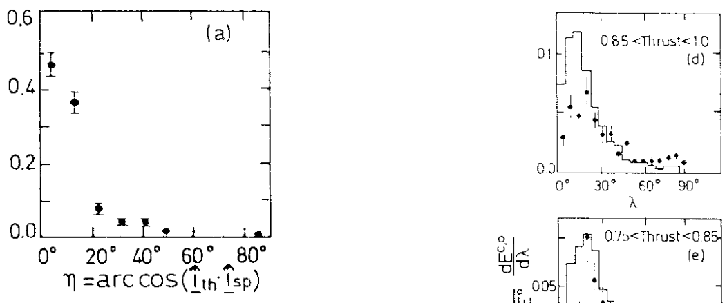
Fig. 12) Distribution of the angle \eta between the thrust and sphericity axes at 9.4 GeV from PLUTO 42 .
