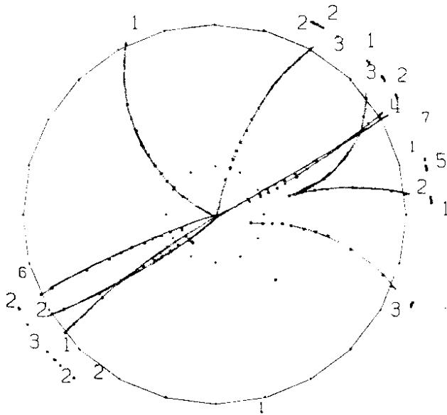
Fig. 14) A jet event from PLUTO taken at E_{CM} = 9.3 GeV (view along the beam). The numbers are shower counter pulse heights, measuring the neutral energy (plus part of the charged energy).
