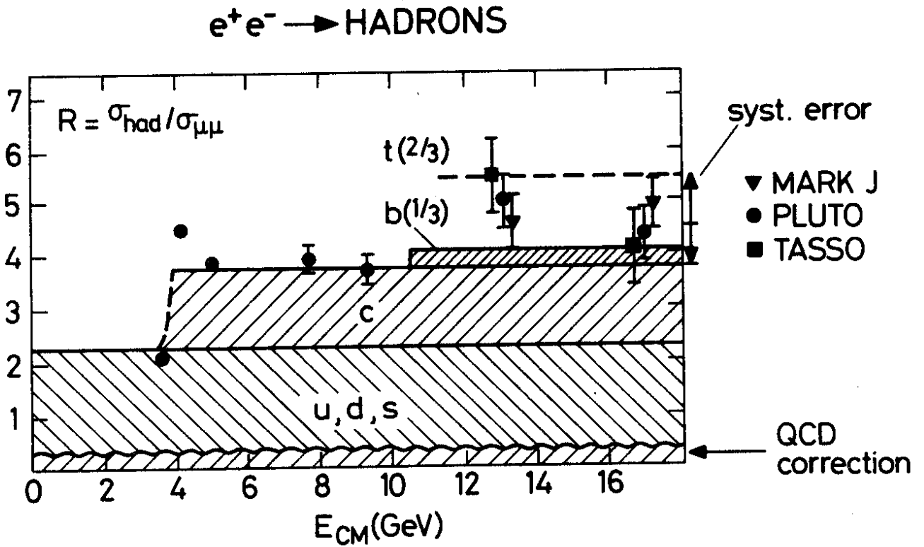
Fig. 59 PLUTO, TASSO, MARK J: measurement of R = \sigma_{\text{had}}/\sigma_{\mu\mu} at 13 and 17 GeV. The PLUTO data below 10 GeV are given for comparison. The expectations for different flavours are indicated.
