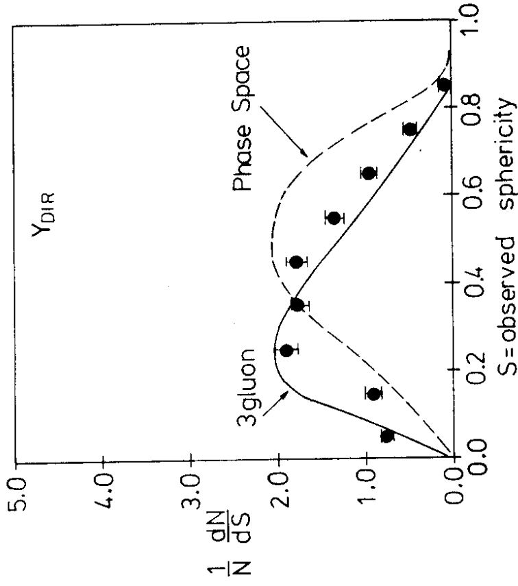
Fig. 34 PLUTO: (preliminary) observed S distributions at 9.4 GeV. b) ON resonance: curves as in fig. 33
