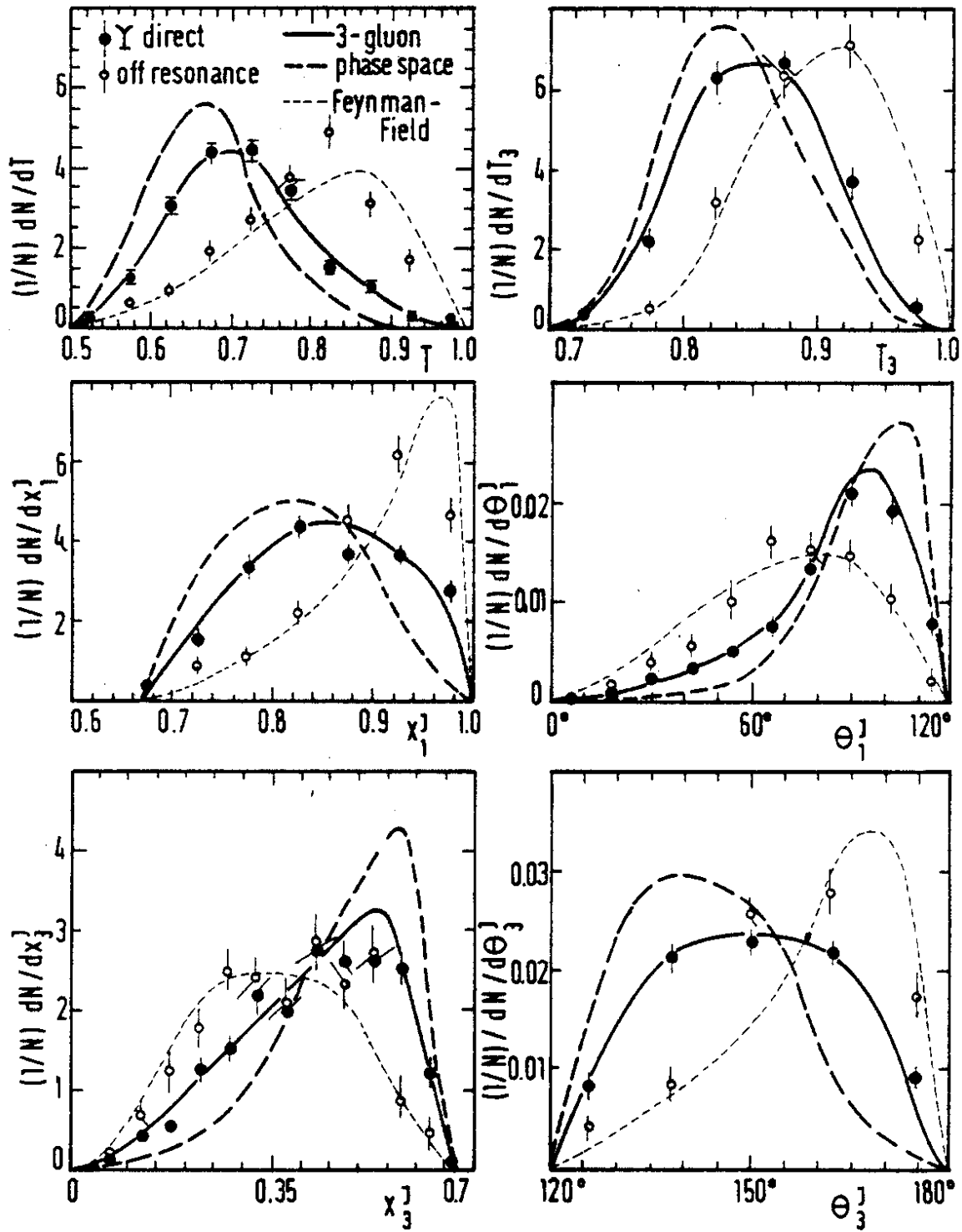
Fig. 2 Experimental distributions of thrust T , triplicity T_3 reconstructed gluon energies x_1^J , x_3^J and reconstructed angles \theta_1^J , \theta_3^J between gluons compared to Monte-Carlo calculations based on various models.
