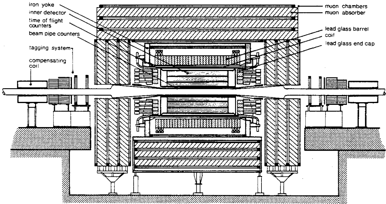
Fig. 1: A sectional view of the JADE detector in a vertical plane containing the beam axis.
