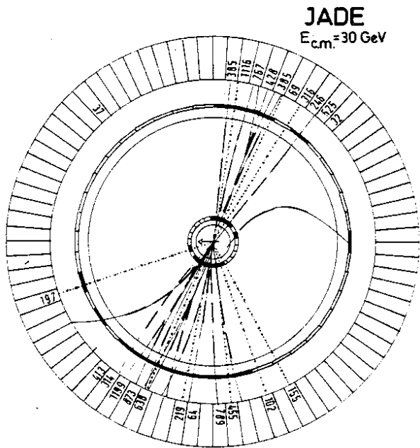
Fig. 2-a: A typical multihadron event (view along the beam) recorded in the central part of the JADE detector. Trajectories of charged and neutral particles are represented by full and dotted lines respectively. The shower counters are also shown here, each wedge representing a row of 30 lead glass counters. The energy deposited in each of these rows appears in units of MeV.
