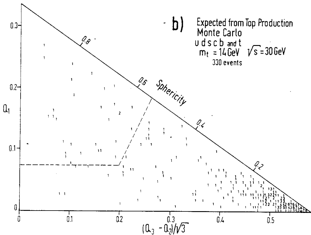
Fig. 9: "Event shape" Q-plots as defined in the text.
