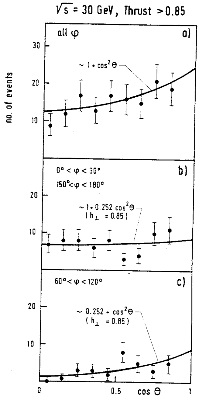
Fig. 19: \cos\theta distribution of the jet axes; a) integrated over all \phi , b) in the \phi region near the horizontal direction, and c) near the vertical direction.
