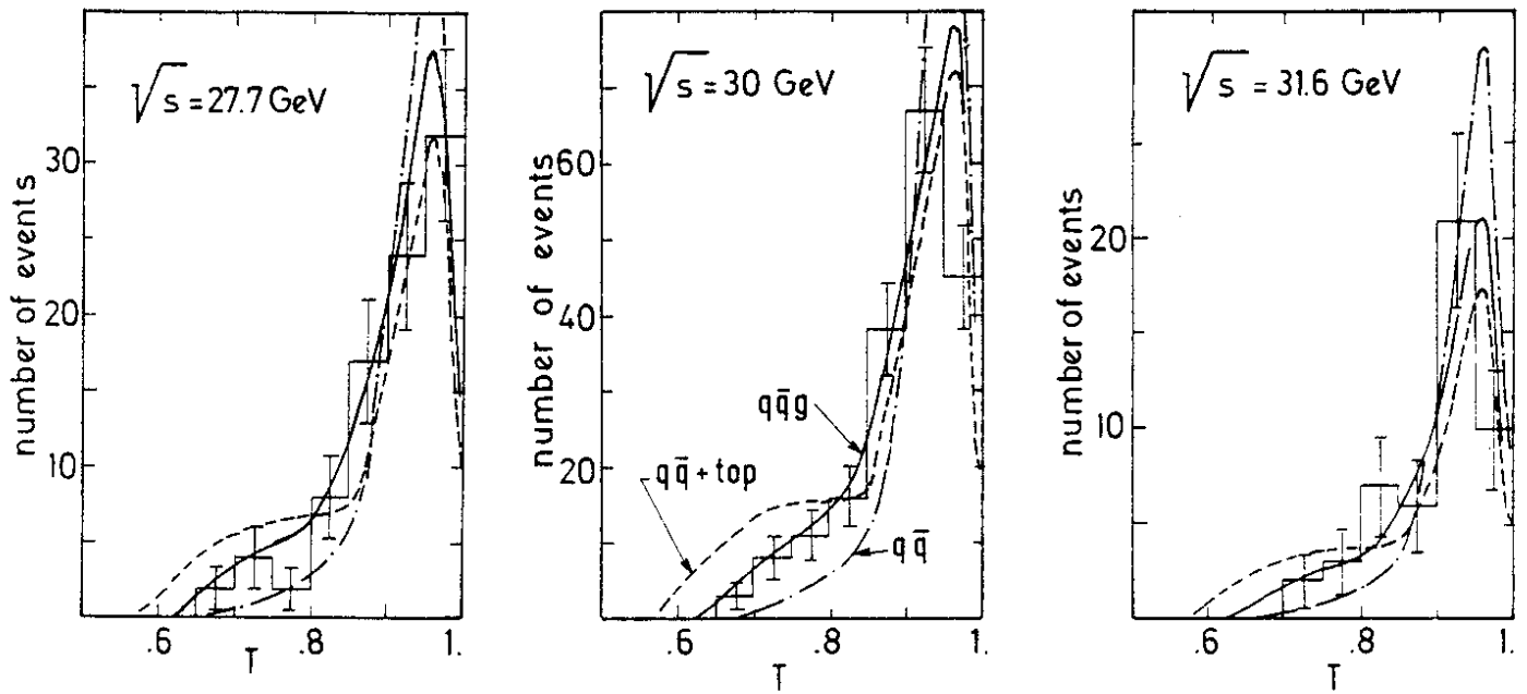
Fig. 10: The thrust distributions at various \sqrt{s} .
