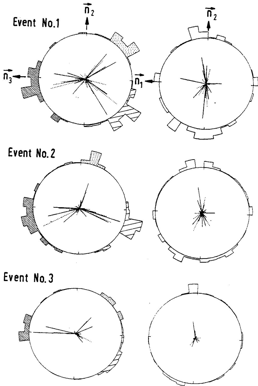
Fig. 14a): Typical three jet events projected onto the (\vec{n}_3, \vec{n}_2) and (\vec{n}_1, \vec{n}_2) planes. The full and dotted lines represent the momentum vectors of charged and neutral particles respectively. The energy flow is shown by the histograms plotted on a circle around each event. The three energy clusters obtained from a three-
