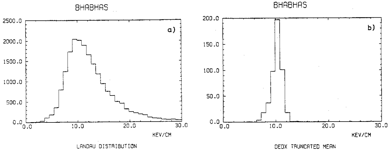
Fig. 15: dE/dx distributions for e^\pm from Bhabha scattering:
