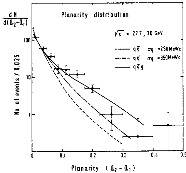
Fig. 13: The planarity distribution compared with model predictions.
