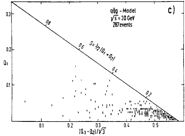
Fig. 12: "Event shape" Q-plot.
