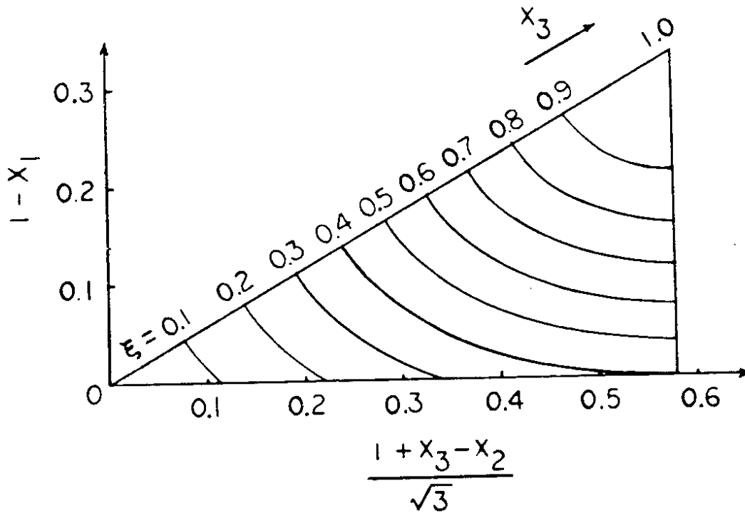
Fig. 4.25(b) The contours of constant z plotted in the (x_1, x_2, x_3) plane.
