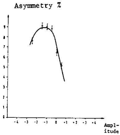
Fig. 4b. As in Fig.4a but for the 38th sine harmonic.
