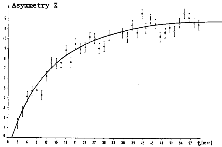
Fig. 2. Exponential build up in time of the polarimeter asymmetry at PETRA at 16.5 GeV
