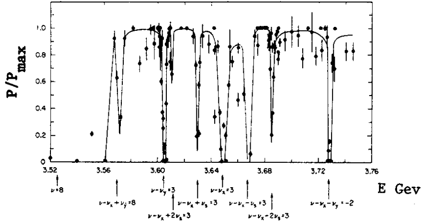
Fig. 3a. Polarization as a function of energy measured at SPEAR. (From Ref. 11)
