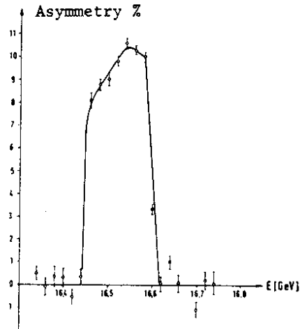
Fig. 4c. Polarimeter asymmetry at PETRA as a function of energy after closed orbit optimisation.
