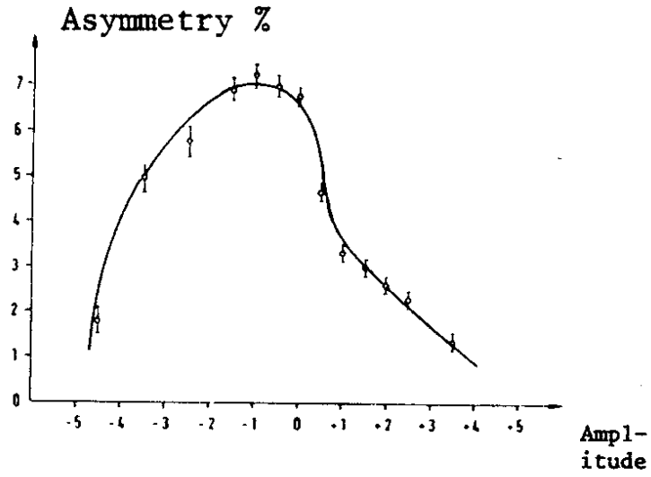
Fig. 4a. Polarimeter asymmetry at PETRA vs. the strength of the 38th cosine harmonic in the closed orbit (arbitrary units).
