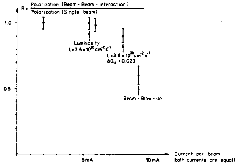
Fig. 5. Ratio of colliding beam polarization to single beam polarization vs. current at PETRA.
