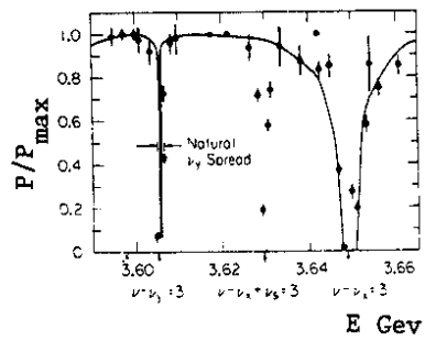
Fig. 3c. Detail of SPEAR polarization curve showing non-linear resonance: a\delta - Q_x + Q_s = 3 (From Ref. 11)
