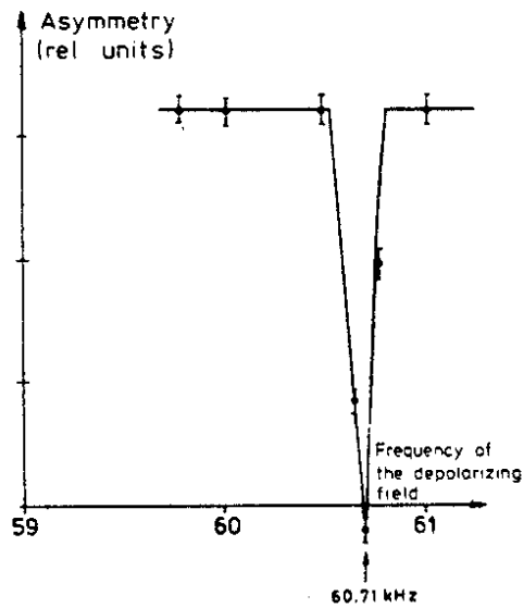
Fig. 6. Polarimeter asymmetry vs. depolarizer frequency at PETRA in the vicinity of 16.5 GeV.
