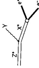
Fig. 12: A composite scalar X^0 mediating radiative Z^0 decays
