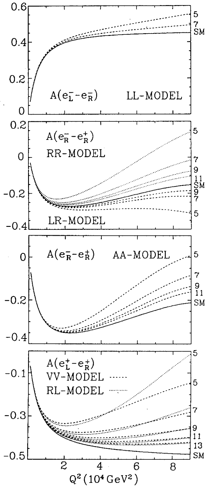
Fig. 5 Expected deviations from the Standard Model predictions (SM) at \sqrt{s} = 1.4 \text{ TeV} and x = 0.05 for various values of \Lambda_{eq} (in \text{TeV} ) and \epsilon = +1 . For each type of contact term the most sensitive asymmetry is plotted.
