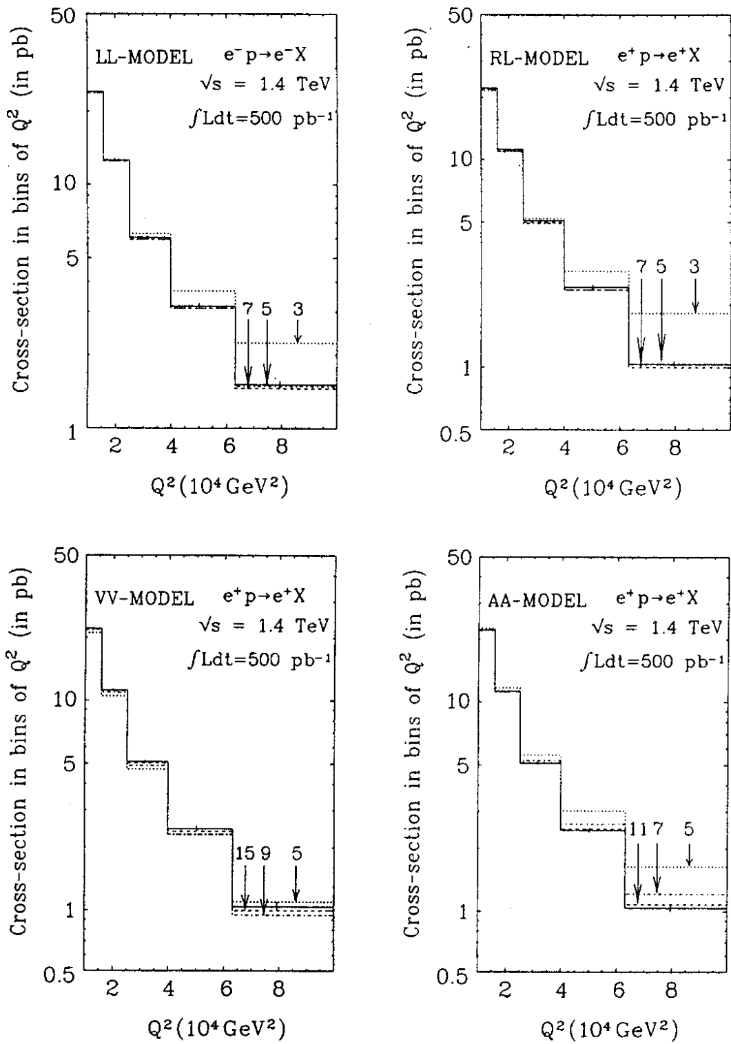
Fig. 2 Same as in Fig. 1 for a different selection of the contact terms and \epsilon = -1 .
