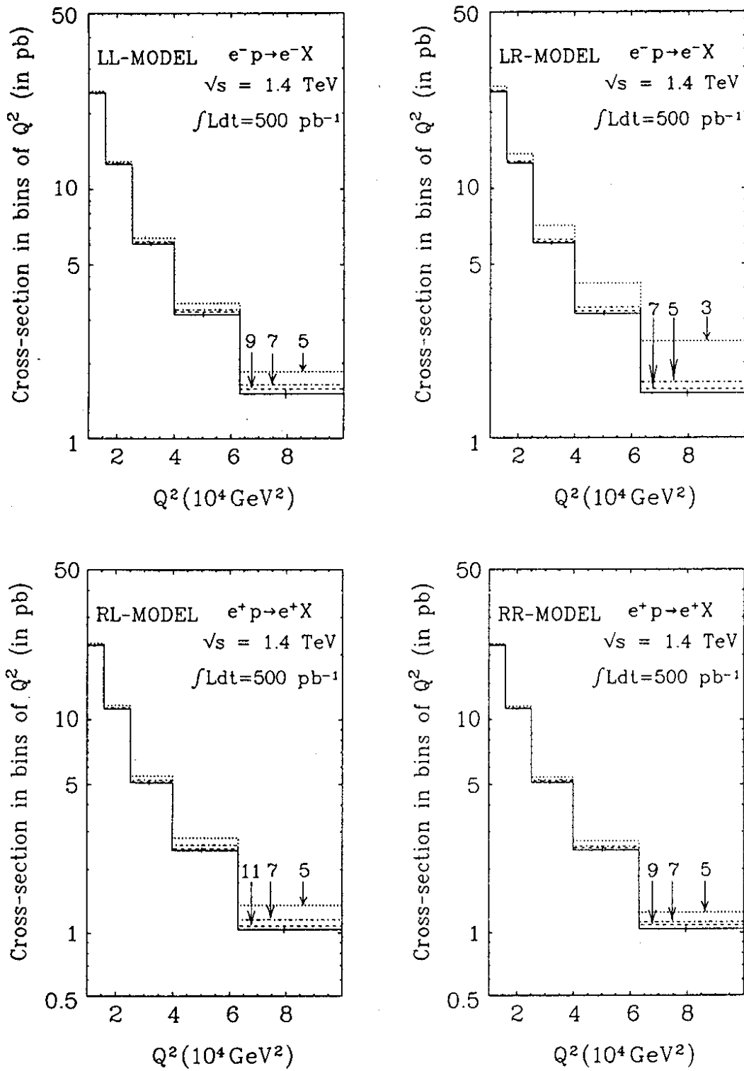
Fig. 1 Neutral current cross-sections integrated over x for contact interactions with \epsilon = +1 in comparison to the Standard Model predictions (full lines). The numbers labelling the curves give the scales \Lambda_{eq} in TeV . The statistical errors refer to a total integrated luminosity of 1fb^{-1} shared equally between e^\mp p collisions.
