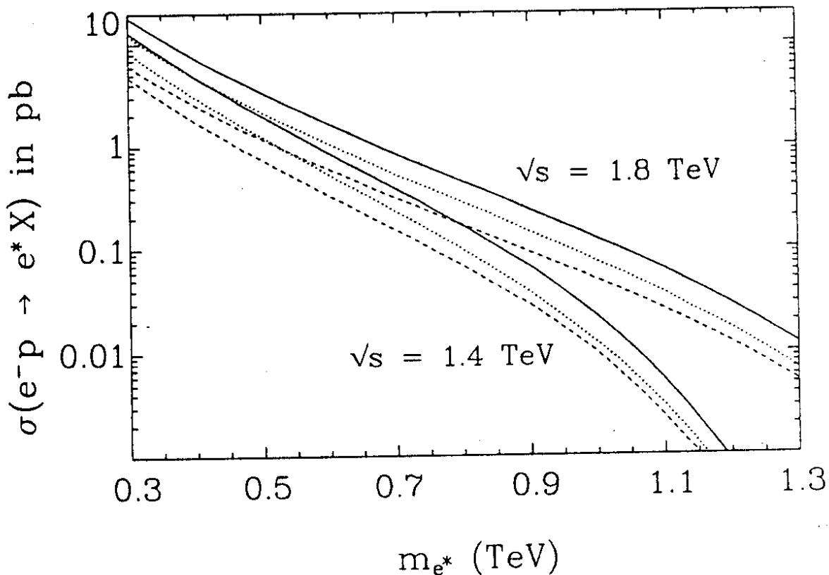
Fig. 7 Excited electron production in ep collisions at LEP-LHC. Shown are the cross-sections for elastic production ep \rightarrow e^*p (dashed), inelastic production ep \rightarrow e^*X (dotted), and the sum of both (full line).
