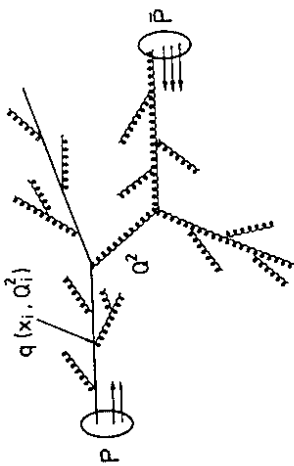
Figure 1: Initial and final state parton radiation in high- p_\perp hadron-hadron scattering.
