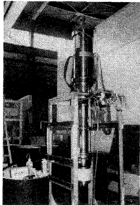
Figure 4. Potograph of prototype klystron.
