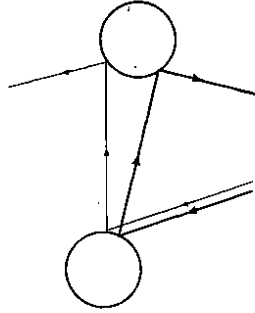
Figure 4: Chaos is sensitive dependence on initial conditions
