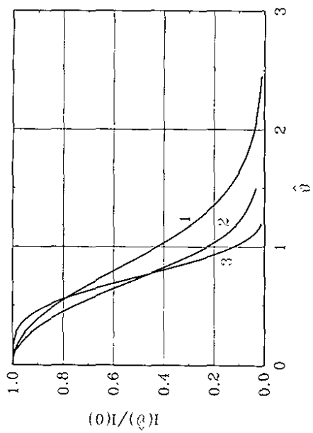
Fig. 11.8. The directivity diagram versus the reduced observation angle: (1): at the linear stage (analytical results), (2): at the saturation, (3): at \hat{z} = 15 with the tapering according to formula (11.6). Here B = 1 , \hat{C} = 0 , \hat{\lambda}_p^2 = 0 , \hat{\lambda}_T^2 = 0 , N = 5 , M = 100 , \hat{w} = 1.2 and \hat{W}_{\text{ext}} = 10^{-3} .
