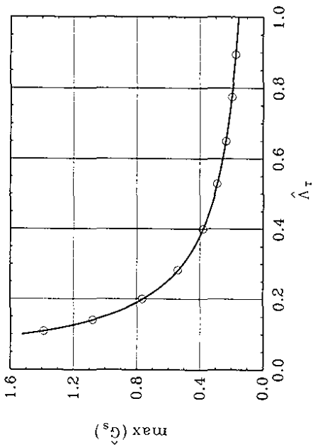
Fig. 8.5. The maximal reduced small-signal gain \hat{G}_s versus the \hat{\Lambda}_T parameter. Here \delta\bar{\psi} = 0 , \hat{l}_1 = 1/2 and \hat{b} = 0 . The full curves is the result of calculations with formula (8.9) and the circles are the result of calculations with asymptotic formula (8.11b).
