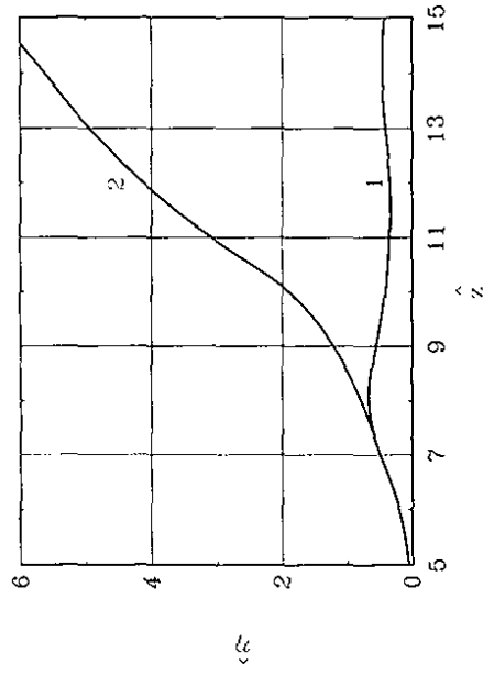
Fig. 11.2. The reduced efficiency \hat{\eta} versus the interaction length. Here B = 1, \hat{C} = 0, \hat{\Lambda}_p^2 = 0, \hat{\Lambda}_t^2 = 0, N = 5, M = 100, \hat{w} = 1.2 and W_{ex} = 10^{-3} . Curve (1): without tapering and curve (2): the tapering according to formula (11.6).
