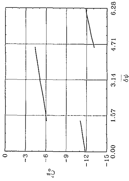
Fig. 8.9. Optimal reduced detuning \hat{C}_0^m versus the \overline{\delta\psi} parameter. Here \hat{d} = 0.3 , \hat{l}_1 = 0.05 , \hat{b} = 30 and \hat{\Lambda}_p^2 = 0 . The calculations have been performed with formula (8.9).
