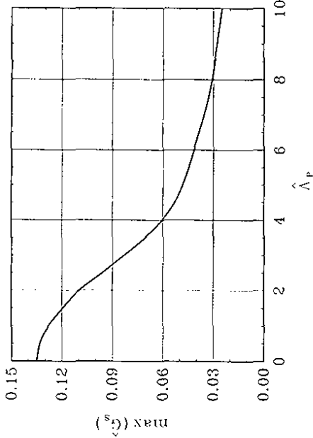
Fig. 5.5. The maximal reduced small-signal gain \hat{G}_s versus the space charge parameter \hat{A}_p at \hat{A}_T^2 = 0 . The calculations have been performed with the formulae (5.3b) and (5.5).
