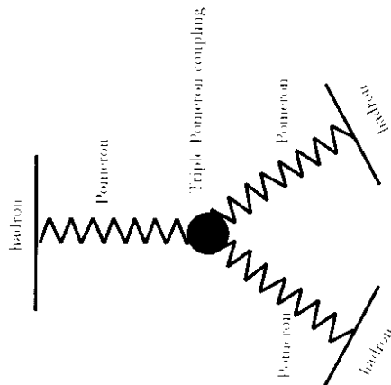
Figure 1.2: Triple Pomeron diagram
