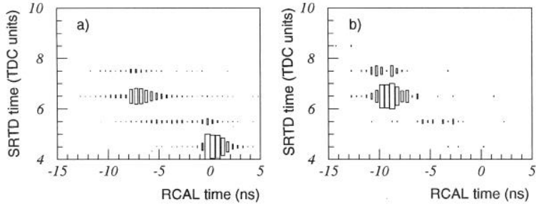
Fig. 15. Scatter plot of SRTD FLT time (TDC units) vs. RCAL time (ns) for a) all events, and b) events dominated by proton-gas background.
