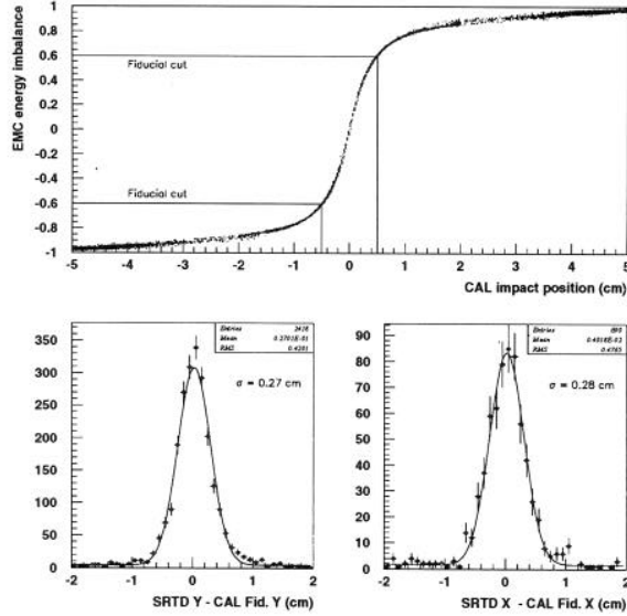
Fig. 12. Electron position measurement. RCAL cell energy imbalance vs. electron impact position (top). Distributions of the SRTD-CAL Y and X positions reconstructed within the fiducial boundary region between two RCAL cells (bottom).
