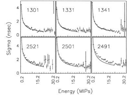
Fig. 9. Single strip timing resolution for a sample of strips measured using DIS data with an electron hit in the SRTD.
