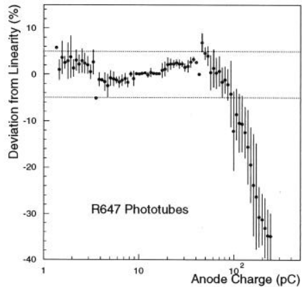
Fig. 7. The average nonlinearity of a sample of R647 PMTs as a function of anode charge. The error bars indicate the spread in nonlinearity among the PMTs.
