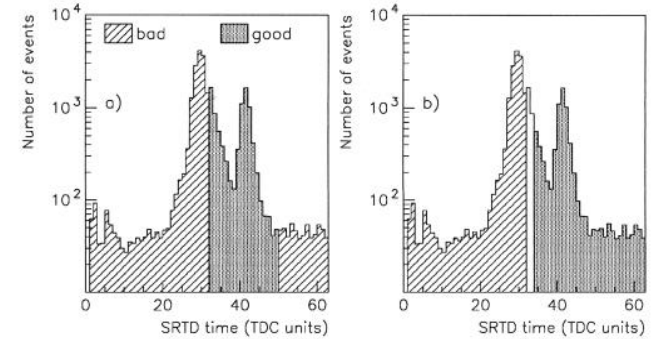
Fig. 16. Unbiased SRTD FLT timing spectrum in the 1995 run. The peak around 30 TDC units is due to proton beam-gas events, while the peak around 40 TDC units is due to ep events. The two different definitions of good and bad timing used in 1995 are illustrated.
