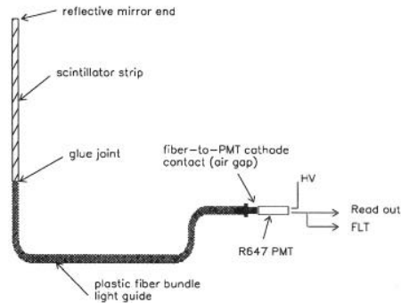
Fig. 4. A schematic layout for one SRTD detector channel (not to scale).
