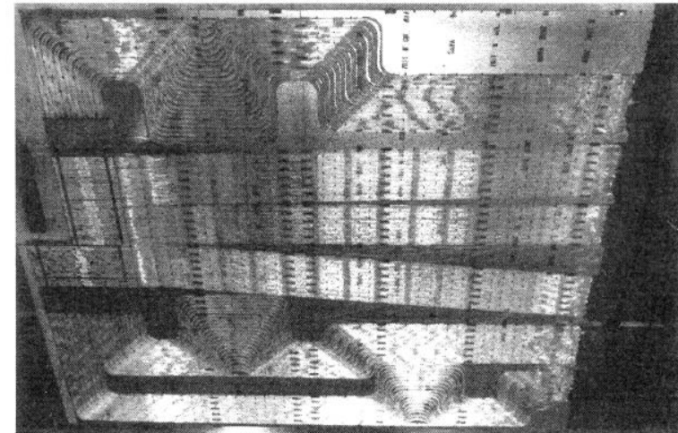
Fig. 5. A photograph of one half of the SRTD with the top cover removed. The layer of horizontal strips is visible near the center-left. The vertical strips are situated beneath the horizontal ones. Also shown are the light guides grouped into equal lengths leading from the strips to the PMTs (not shown) located along the right-edge of the support structure.
