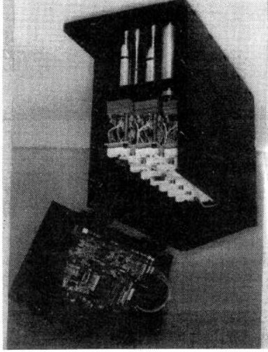
Fig. 6. A photograph of the PMT box. A side plate has been removed and the lid opened to show clearly the interior layout. The PMTs are shown facing downwards in the picture.
