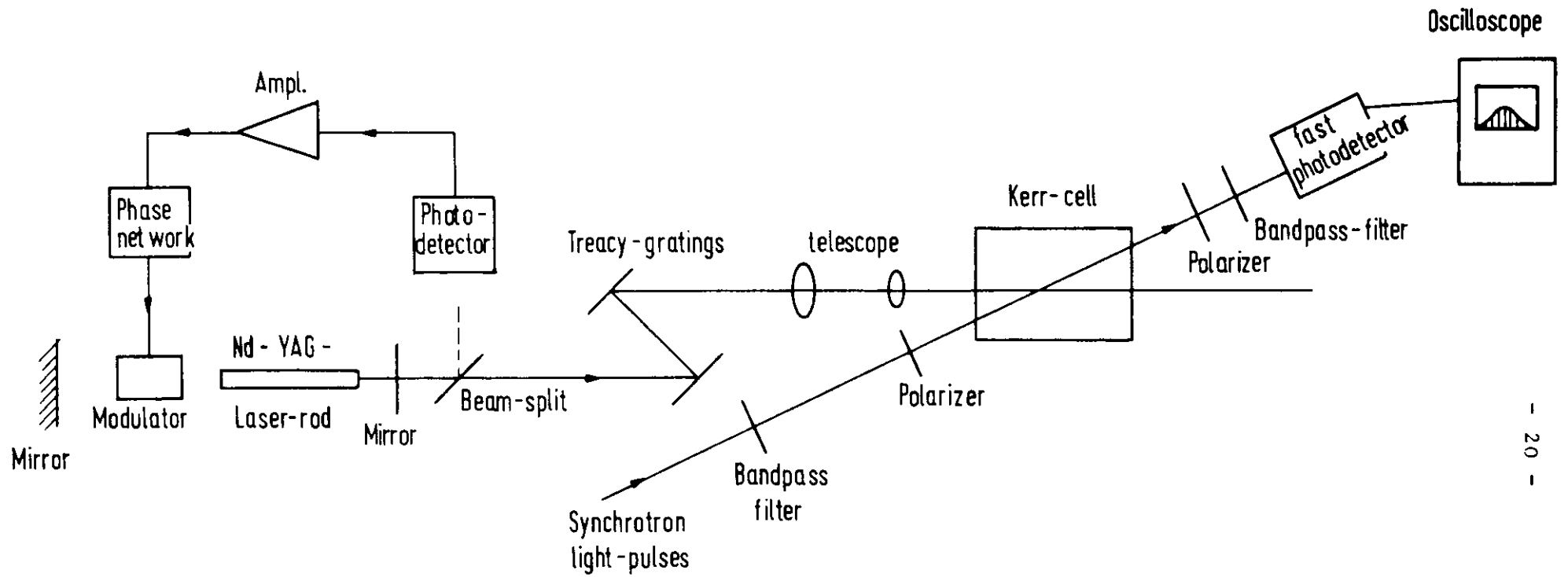
fig.20 : Final apparatus for measuring synchrotron pulses in the picosecond range
