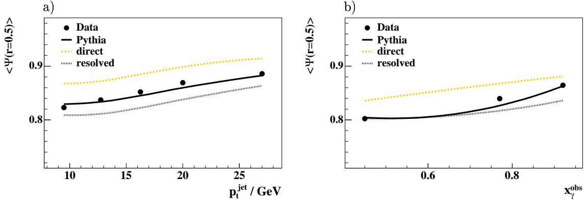
Figure 5.13: Mean integrated jet shape at fixed radius r = 0.5 for the flavour inclusive dijet sample as functions of a) p_t^{\text{jet}} and b) the observable x_\gamma^{\text{obs}} . The statistical errors in both data and Monte Carlo simulation are negligible. Smooth curves connect the Monte Carlo predictions which are measured at the same points as the data.
