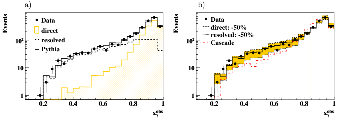
Figure 7.3: Distributions of the variable x_\gamma^{obs} for the heavy flavour enriched sample (see section 6.6). The Monte Carlo distributions are normalised to match the data. Contributions from direct and resolved processes are shown separately for the default PYTHIA in figure a). Variations of the relative fractions of direct and resolved processes lead to the uncertainty band (shaded region) in figure b). Cascade (dashed-dotted line) is shown separately.
