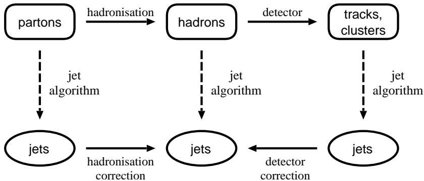
Figure 4.11: Schematic diagram of the parton, hadron and detector level jets. At each different stage the jet finding algorithm can be applied which is used to compare detected data with parton level calculations.
