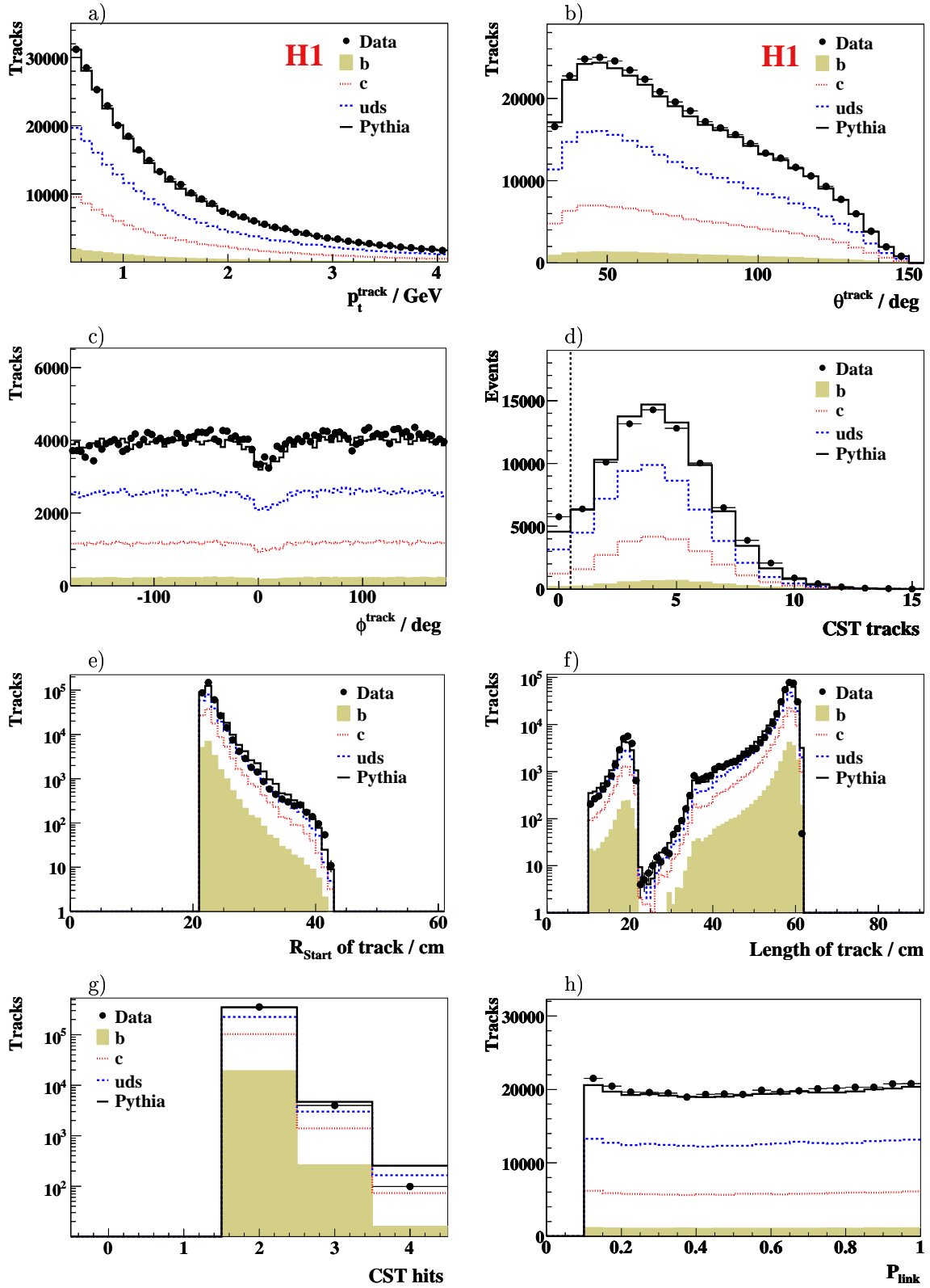
Figure 6.1: Control distributions of the selected tracks. The expectation from the PYTHIA Monte Carlo simulation is included in the figure, showing the contributions from the various quark flavours after applying the scale factors obtained from the fit to the subtracted significance distributions of the data (see section 6.3).
