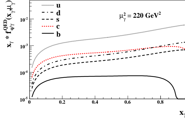
Figure 2.6: Quark density of the photon (QED result).
