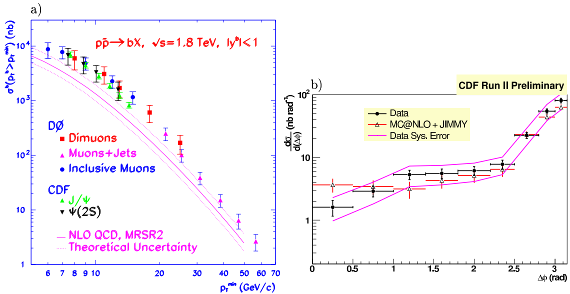
Figure 3.10: TEVATRON Run I and Run II results for beauty quark production. a) A collection of D0 and CDF beauty measurements. b) A recent b\bar{b} jets measurement performed by CDF. The data is compared to the prediction from the MC@NLO generator.
