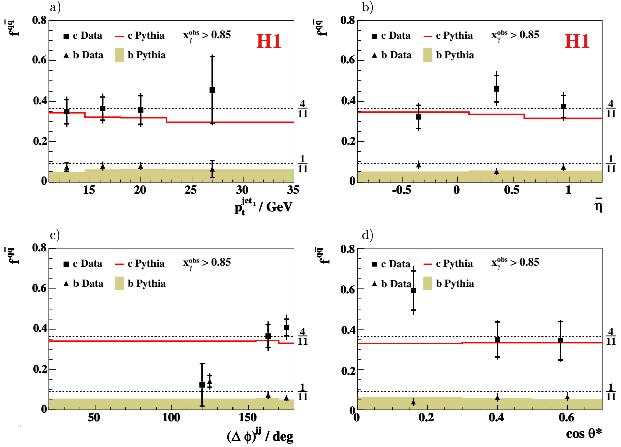
Figure 7.14: Relative contributions from charm (squares) and beauty events (triangles) as a function of a) the transverse momentum of the leading jet p_t^{jet_1} , b) the mean pseudo-rapidity \bar{\eta} , c) the azimuthal distance of the two jets (\Delta\phi)^{jj} and d) the variable \cos\theta^* for the region x_\gamma^{obs} > 0.85 . The inner error bars indicate the statistical uncertainty and the outer error bars show the statistical and systematic error added in quadrature. The solid line (shaded area) indicates the absolute prediction from PYTHIA for charm (beauty). The dashed lines correspond to the absolute predictions from naïve quark charge counting.
