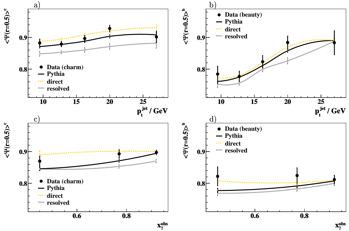
Figure 6.13: Mean integrated jet shape at fixed radius r = 0.5 for the heavy quark enriched dijet sample as functions of a), b) p_t^{\text{jet}} and c), d) the observable x_\gamma^{\text{obs}} . The left (right) column shows the charm (beauty) data after background subtraction (see text). The data is compared to the total charm and beauty PYTHIA predictions (full line). Direct (dashed line) and resolved (dotted line) contributions are shown separately. Only statistical errors are shown.
