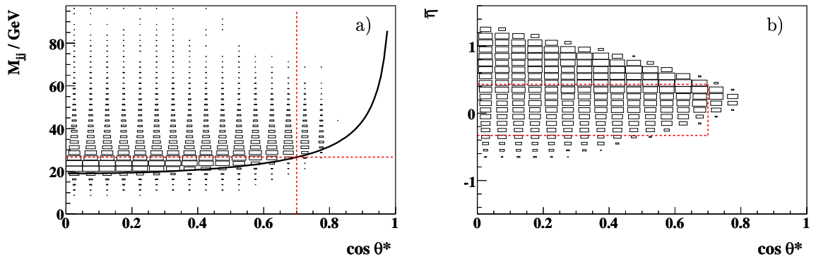
Figure C.1: Correlations of the scattering angle \theta^* and a) the invariant mass M_{jj} , b) the mean pseudo-rapidity \bar{\eta} . The horizontal and vertical dashed lines show the cuts, while the solid curve in a) corresponds to equation C.2 for jet transverse momenta p_t^{jet} > 11 GeV.
