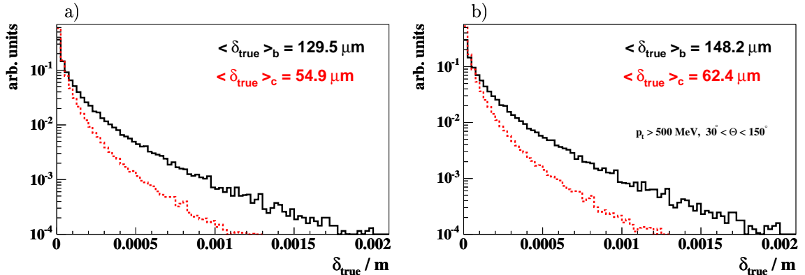
Figure 4.2: Normalised distributions of the true track impact parameter \delta_{true} for charm (dotted) and beauty (full) events calculated with PYTHIA; a) without cuts and b) for tracks with p_t > 500 \text{ MeV} in the angular acceptance range of the CST.
