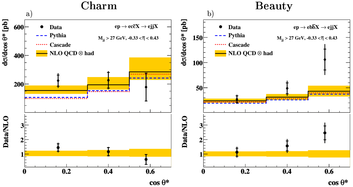
Figure 7.8: Differential charm and beauty photoproduction cross sections a, b) d\sigma/d\cos\theta^* for the process ep \rightarrow e(c\bar{c} \text{ or } b\bar{b})X \rightarrow ejjX . The inner error bars indicate the statistical uncertainty and the outer error bars show the statistical and systematic errors added in quadrature. The solid lines indicate the prediction from a massive NLO QCD calculation, corrected for hadronisation effects, and the shaded band shows the estimated uncertainty. The absolute predictions from PYTHIA (dashed lines) and CASCADE (dotted lines) are also shown.
