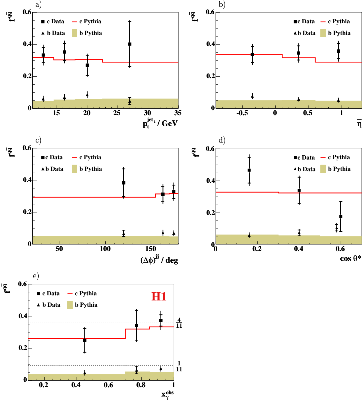
Figure 7.13: Relative contributions from charm (squares) and beauty events (triangles) as a function of a) the transverse momentum of the leading jet p_t^{\text{jet}_1} , b) the mean pseudo-rapidity \bar{\eta} , c) the azimuthal distance of the two jets (\Delta\phi)^{jj} , d) the observable \cos\theta^* and e) the observable x_\gamma^{\text{obs}} . The inner error bars indicate the statistical uncertainty and the outer error bars show the statistical and systematic error added in quadrature. The solid line (shaded area) indicates the absolute prediction from PYTHIA for charm (beauty). The dashed lines in figure e) correspond to the absolute predictions from naïve quark charge counting.
