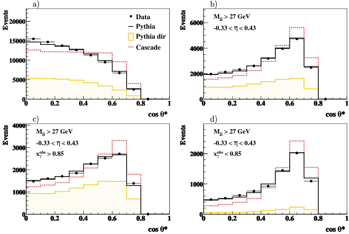
Figure C.2: Distributions of the scattering angle \theta^* for the flavour inclusive dijet sample. The data are compared to the PYTHIA (full line) and CASCADE (dotted line) simulation for a) \cos\theta^* b) \cos\theta^* with additional cuts on M_{jj} and \bar{\eta} and for c) direct ( x_\gamma^{obs} > 0.85 ) and d) resolved ( x_\gamma^{obs} < 0.85 ) enriched samples. The Monte Carlo distributions are normalised to the number of events in the data.
