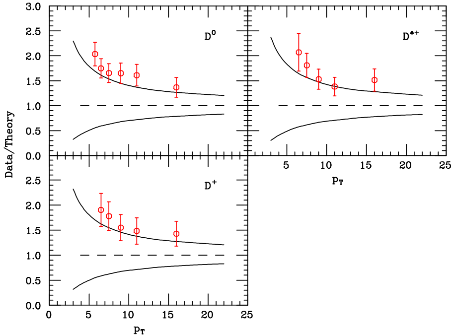
Figure 3.9: CDF Run II results for charm quark production as a function of the transverse momentum of the D-meson. Shown are ratios between the experimental results and the central theoretical predictions obtained with the FONLL approach.
