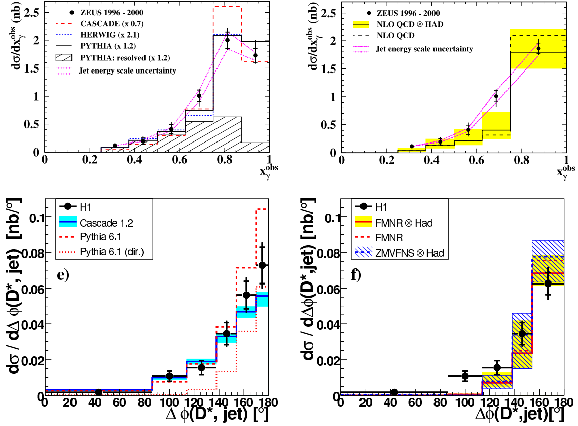
Figure 3.5: Charm dijet measurements at HERA. Top: Differential D^* dijet photoproduction cross section as a function of x_\gamma^{obs} from ZEUS [9]. Bottom: Differential charm cross section as a function of \Delta\phi in a D^* -jet sample from H1 [16].
