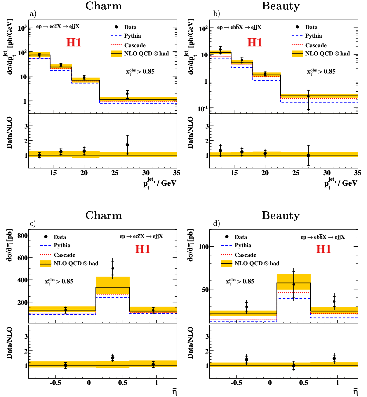
Figure 7.9: Differential charm and beauty photoproduction cross sections a, b) d\sigma/dp_t^{jet1} and c, d) d\sigma/d\eta for the process ep \rightarrow e(c\bar{c} \text{ or } b\bar{b})X \rightarrow ejjX in the region x_\gamma^{obs} > 0.85 . The inner error bars indicate the statistical uncertainty and the outer error bars show the statistical and systematic errors added in quadrature. The solid lines indicate the prediction from a massive NLO QCD calculation, corrected for hadronisation effects, and the shaded band shows the estimated uncertainty. The absolute predictions from PYTHIA (dashed lines) and CASCADE (dotted lines) are also shown.
