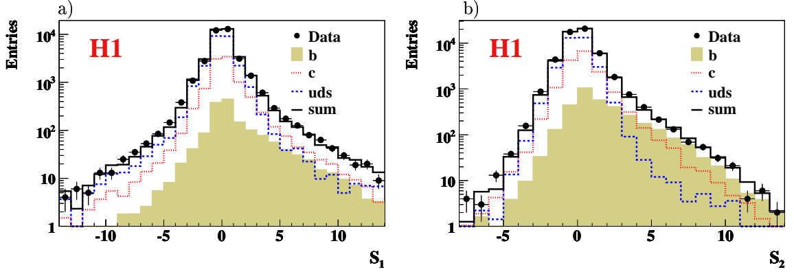
Figure 6.4: Distributions of a) the significance S_1 of tracks in jets with exactly one selected track and b) the significance S_2 of the track with the second highest significance in jets with two or more selected tracks. Only tracks with an impact parameter |\delta| < 0.1 cm are considered. The expectation from the PYTHIA Monte Carlo simulation is included in the figure, showing the contributions from the various quark flavours after applying the scale factors obtained from the fit to the subtracted significance distributions of the data (see section 6.3).
