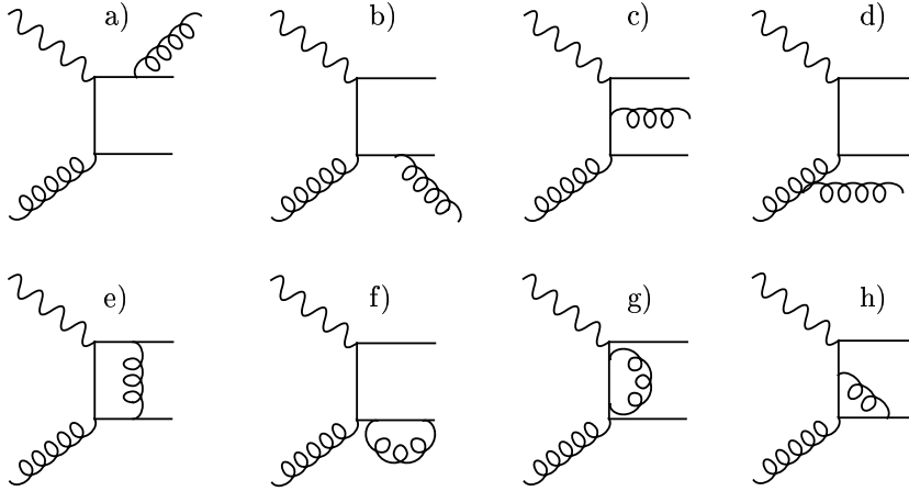
Figure 2.9: Some of the NLO corrections to the BGF process in the massive scheme. a)-d) Gluon radiation, e)-h) virtual corrections.
