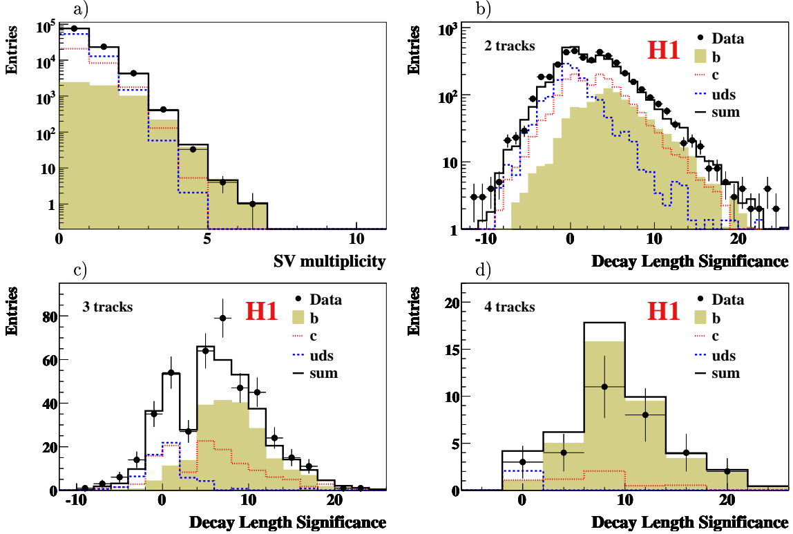
Figure 6.8: Distributions of a) the secondary vertex (SV) multiplicity and the decay length significance ( l/\sigma_l ) with multiplicities SV=2 (b), SV=3 (c) and SV=4 (d). PYTHIA is scaled with the scale factors as obtained from the fit to the subtracted ( S_1, S_2 )-distributions.
