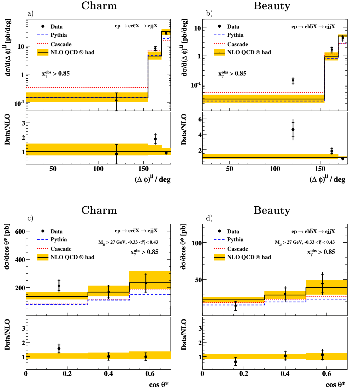
Figure 7.10: Differential charm and beauty photoproduction cross sections a, b) d\sigma/d(\Delta\phi)^{jj} and c, d) d\sigma/d\cos\theta^* for the process ep \rightarrow e(c\bar{c} \text{ or } b\bar{b})X \rightarrow ejjX in the region x_\gamma^{obs} > 0.85 . The inner error bars indicate the statistical uncertainty and the outer error bars show the statistical and systematic errors added in quadrature. The solid lines indicate the prediction from a massive NLO QCD calculation, corrected for hadronisation effects, and the shaded band shows the estimated uncertainty. The absolute predictions from PYTHIA (dashed lines) and CASCADE (dotted lines) are also shown.
