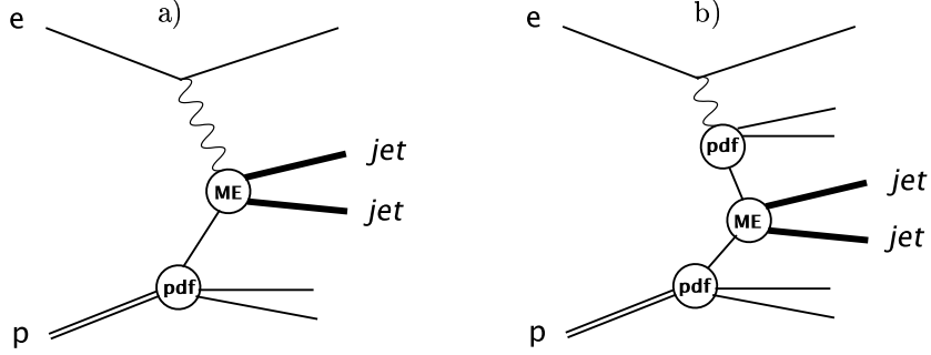
Figure 2.5: a) Direct and b) resolved photoproduction of jets in leading order.
