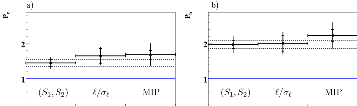
Figure 6.9: Summary of the results from the independent quark flavour separation methods. Shown are the scale factors P_c (a) and P_b (b) as obtained from the fit to the subtracted (S_1, S_2) -distributions, the fit to the decay length significance (\ell/\sigma_\ell) distributions and the fit to the multi-impact parameter (MIP) distribution. The inner error bars indicate the statistical uncertainty and the outer error bars show the statistical and systematic error added in quadrature.
