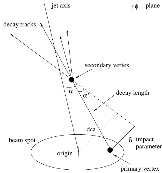
Figure 4.1: Schematic illustration of the impact parameter in the r\phi -plane.
