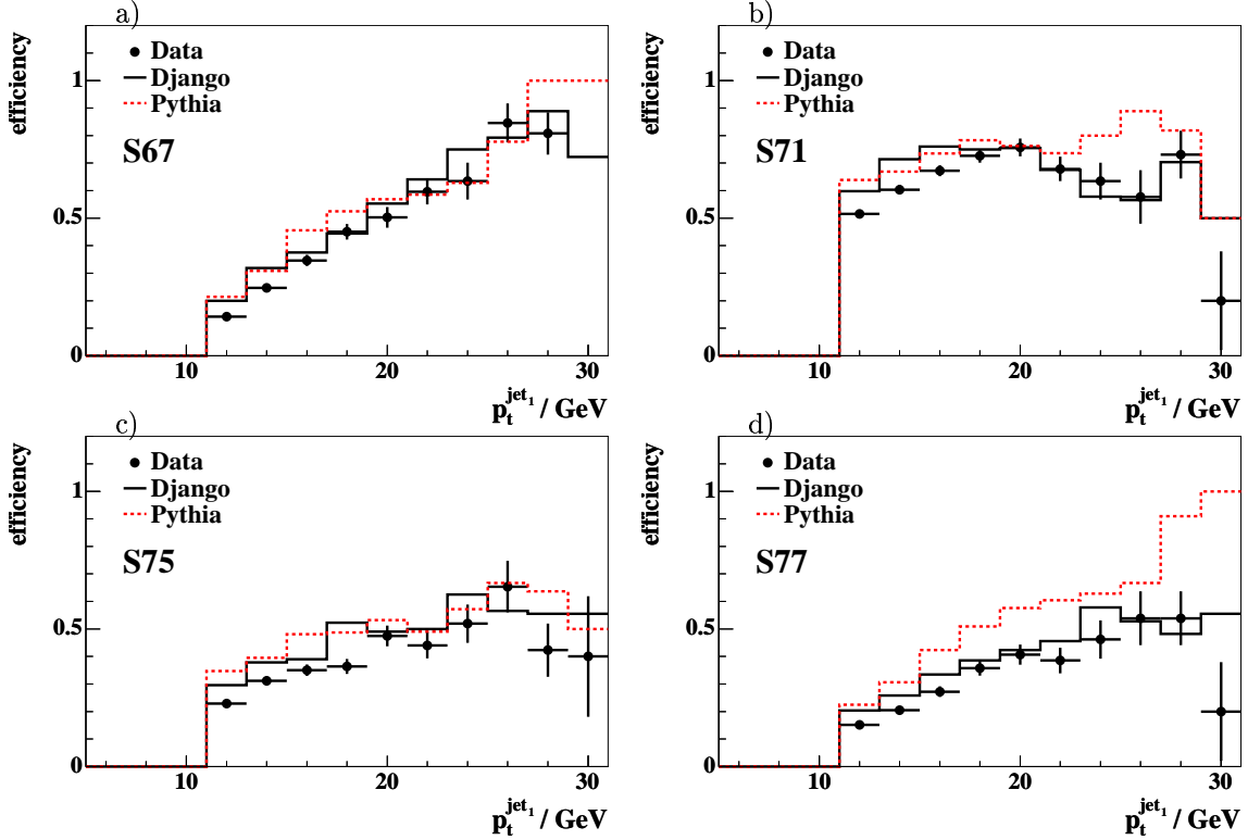
Figure 5.3: The trigger efficiency for the individual signal triggers as a function of the transverse momentum of the leading jet before correction.
