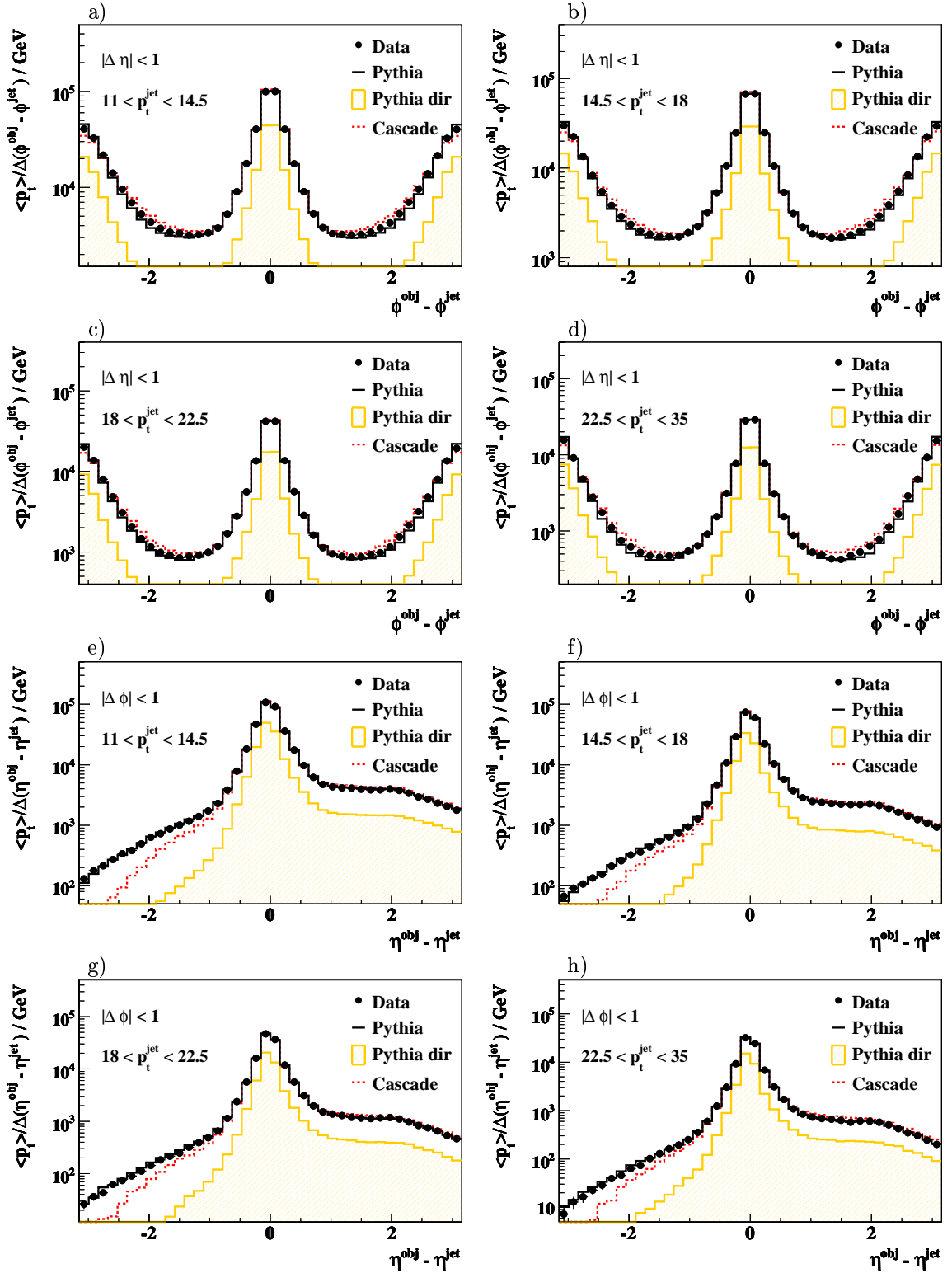
Figure 5.12: The transverse energy flow around the jet axis as a function of the distance to the jet axis in azimuthal angles \phi^{obj} - \phi^{jet} (a-d) and as a function of the distance in pseudo-rapidity \eta^{obj} - \eta^{jet} (e-h) for different p_t^{jet} regions.
