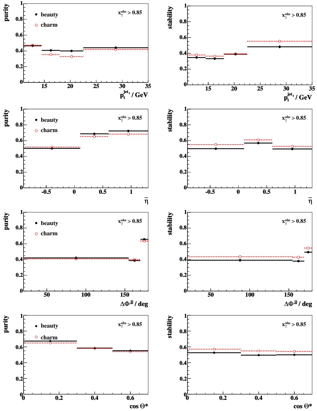
Figure 5.16: Purities and Stabilities for the chosen bins in p_t^{\text{jet}_1} , \bar{\eta} , (\Delta\phi)^{jj} and \cos\theta^* in the region x_\gamma^{\text{obs}} > 0.85 . The full (open) points show the values obtained with the beauty (charm) PYTHIA Monte Carlo simulation.
