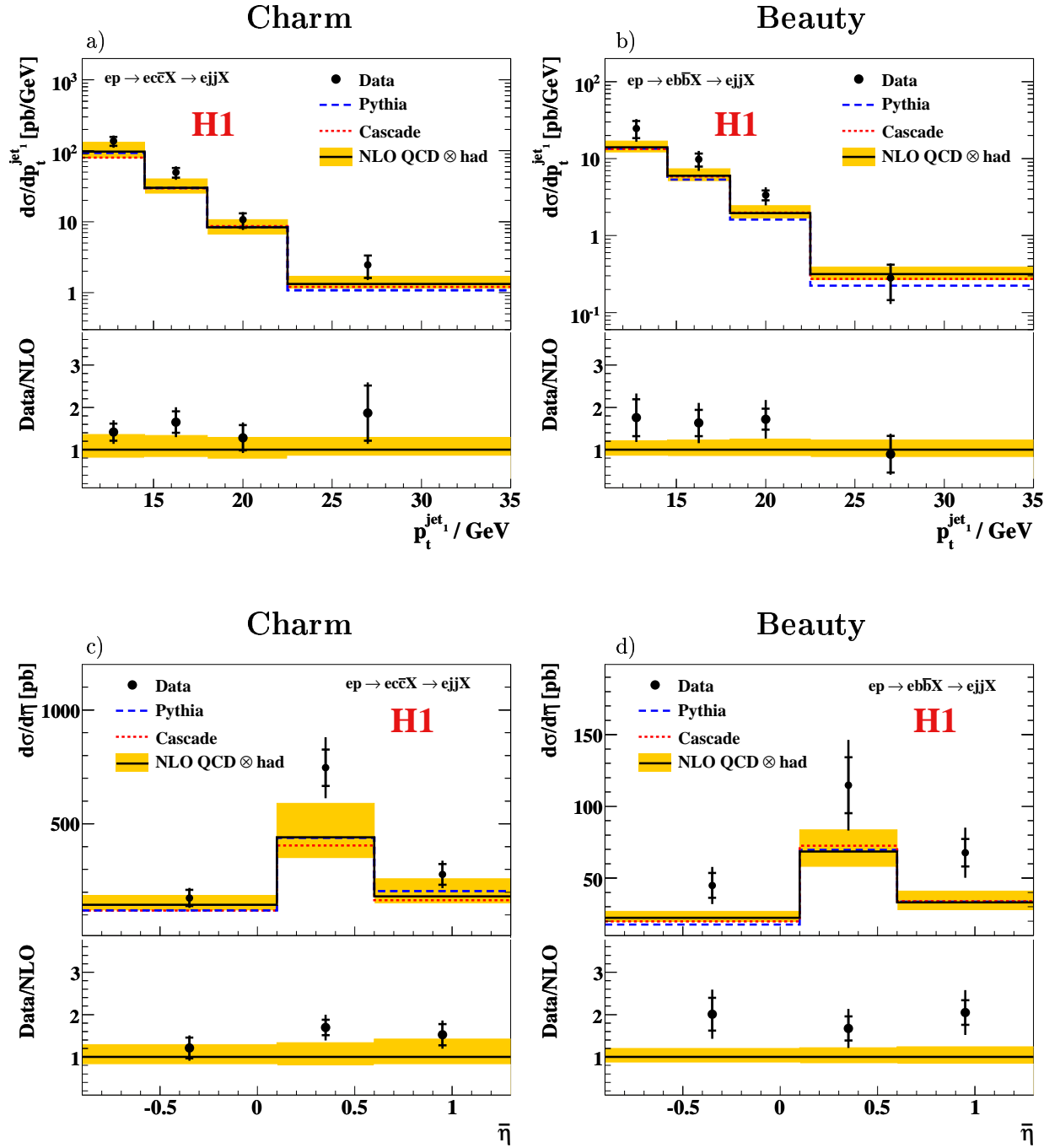
Figure 7.6: Differential charm and beauty photoproduction cross sections a, b) d\sigma/dp_t^{jet1} and c, d) d\sigma/d\eta for the process ep \rightarrow e(c\bar{c} \text{ or } b\bar{b})X \rightarrow ejjX . The inner error bars indicate the statistical uncertainty and the outer error bars show the statistical and systematic errors added in quadrature. The solid lines indicate the prediction from a massive NLO QCD calculation, corrected for hadronisation effects, and the shaded band shows the estimated uncertainty. The absolute predictions from PYTHIA (dashed lines) and CASCADE (dotted lines) are also shown.
