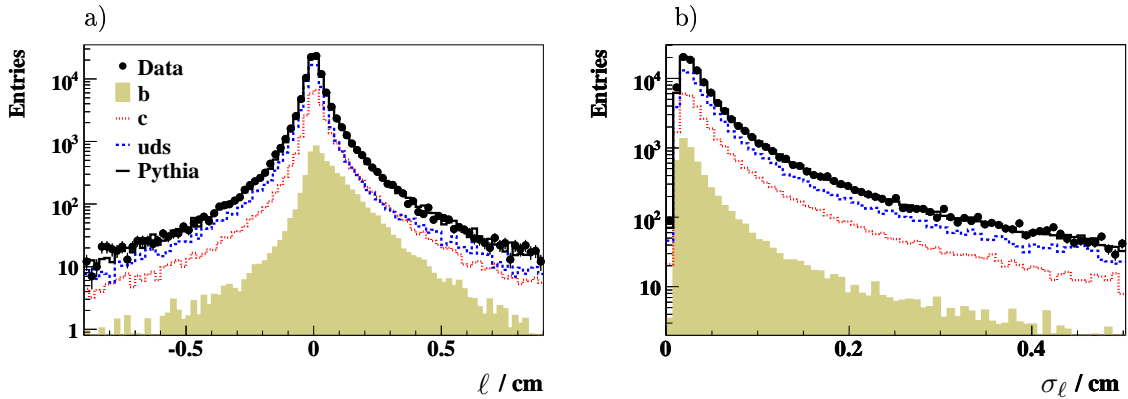
Figure 6.7: Distributions of a) the decay length \ell and b) the decay length error \sigma_\ell for both jets. For the secondary vertex only tracks with an impact parameter |\delta| < 0.1 cm are chosen. PYTHIA is scaled with the scale factors as obtained from the fit to the subtracted ( S_1 , S_2 )-distributions.
