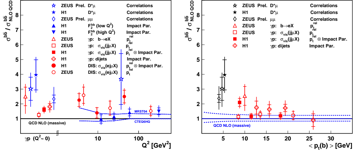
Figure 7.15: Summary of beauty measurements at HERA. The left plot shows the ratio of the cross sections to the (massive) NLO predictions as a function of Q^2 . On the right the dependence on the mean transverse momentum of the b -quark is shown. The results of this analysis are represented by the open crosses.
