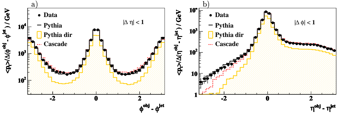
Figure 6.11: The transverse energy flow around the jet axis for the heavy quark enriched sample as a function of a) the distance to the jet axis in azimuthal angles \phi^{obj} - \phi^{jet} and b) as a function of the distance in pseudo-rapidity \eta^{obj} - \eta^{jet} . The predictions from PYTHIA and CASCADE are normalised to the data and indicated as full line and dotted line respectively.
