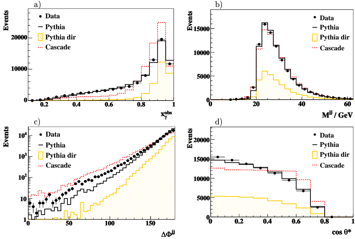
Figure 5.8: Distributions of the two leading jets in the selected dijet sample. The data are compared to the PYTHIA (full line) and CASCADE (dotted line) simulation for the distributions of a) the observable x_{\gamma}^{obs} , b) the invariant dijet mass M^{jj} , c) the azimuthal difference (\Delta\phi)^{jj} of the two jets and d) the observable \cos\theta^* . The Monte Carlo distributions are normalised to the number of events in the data.
