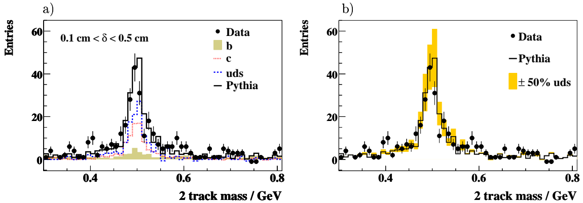
Figure 7.2: Distribution of the invariant 2 track mass in a strangeness enhanced data sample after background subtraction. Events with negative or positive impact parameter significance enter with a weight w = -1 or w = +1 , respectively. In figure a) the data is compared to the PYTHIA simulation. The decomposition into beauty, charm and light quarks is shown separately. In figure b) the same data is shown and compared to modified PYTHIA predictions in which the relative fraction of uds events is varied. The error band of \pm 50\% accounts for the uncertainty in the light quark description of the simulation.
