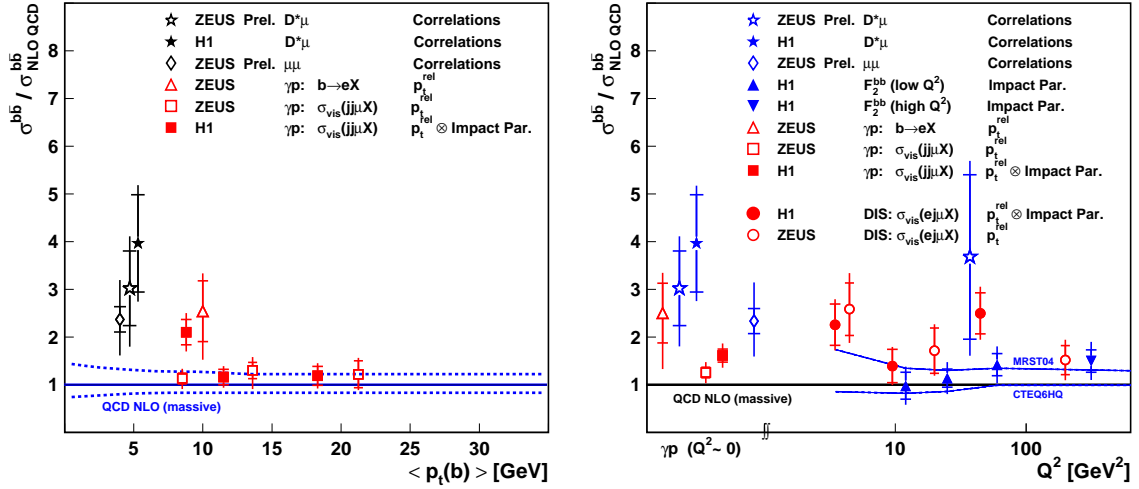
Figure 3.7: Summary of beauty measurements at HERA. The left plot shows the ratio of the cross sections to the NLO predictions as a function of the mean transverse momentum of the b -quark. On the right the dependence on Q^2 is shown.
