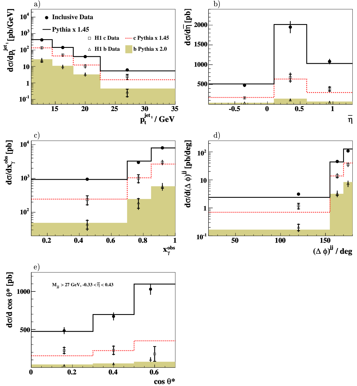
Figure 7.11: Differential flavour inclusive photoproduction cross sections a) d\sigma/dp_t^{\text{jet}_1} , b) d\sigma/d\bar{\eta} , c) d\sigma/dx_\gamma^{\text{obs}} , d) d\sigma/d(\Delta\phi)^{jj} and e) d\sigma/d\cos\theta^* for the process ep \rightarrow eq\bar{q}X \rightarrow ejjX . The inner error bars indicate the statistical uncertainty and the outer error bars show the statistical and systematic errors added in quadrature. The solid lines indicate the absolute prediction from PYTHIA scaled with a factor 1.45. The charm (boxes) and beauty (triangles) data are also shown together with the charm and beauty PYTHIA prediction scaled with the factors P_c = 1.45 and P_b = 2.0 .
