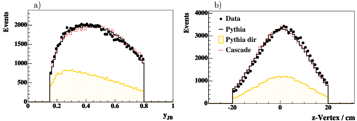
Figure 5.9: Comparison of the dijet data with PYTHIA and CASCADE. Shown are event-normalised distributions of a) the inelasticity y_{JB} and b) the z position of the vertex.
