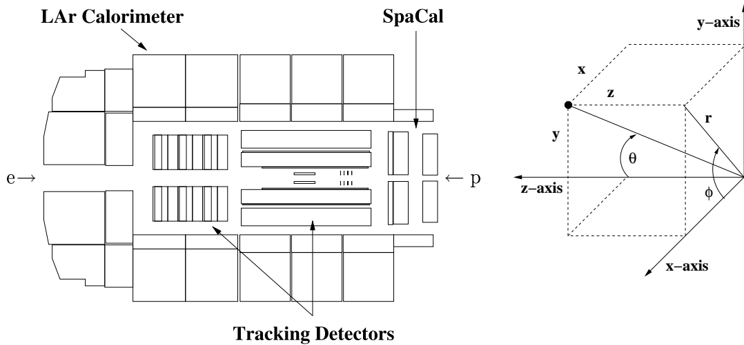
Figure 3.1: Schematic longitudinal section of the H1 detector. Only the most important components used in this analysis are shown. The H1 coordinate system is shown on the right.
