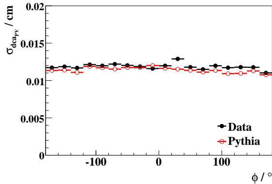
Figure 4.10: Gaussian width of the dca_{PV} distribution as a function of the track direction around the primary vertex. Inclusive tracks with at least two CST hits and p_t > 0.5 \text{ GeV} are shown for data and simulation.
