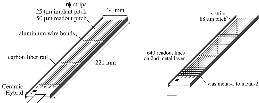
Figure 3.3: CST half ladders: p -side (left) and n -side (right).
