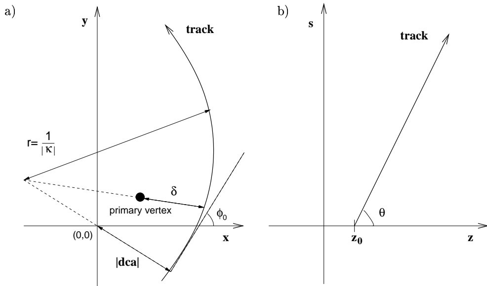
Figure 4.4: The track parameters (\kappa, \phi_0, \theta, dca, z_0) describe the helix in a) the r\phi and b) the zs plane with respect to the origin of the H1 coordinate system.
