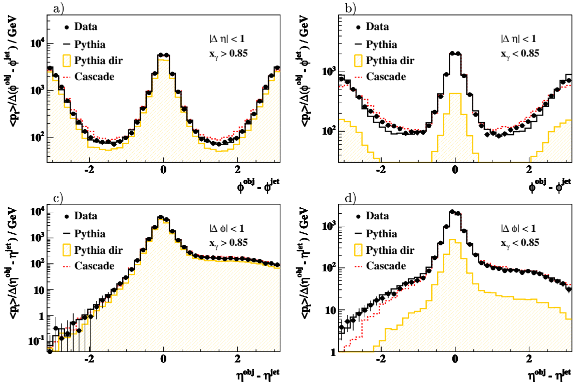
Figure 6.12: The transverse energy flow around the jet axis for the heavy quark enriched sample as a function of a), b) the distance to the jet axis in azimuthal angles \phi^{obj} - \phi^{jet} and c), d) as a function of the distance in pseudo-rapidity \eta^{obj} - \eta^{jet} for different x_\gamma^{obs} regions. The predictions from PYTHIA and CASCADE are normalised to the data and indicated as full line and dotted line respectively.
