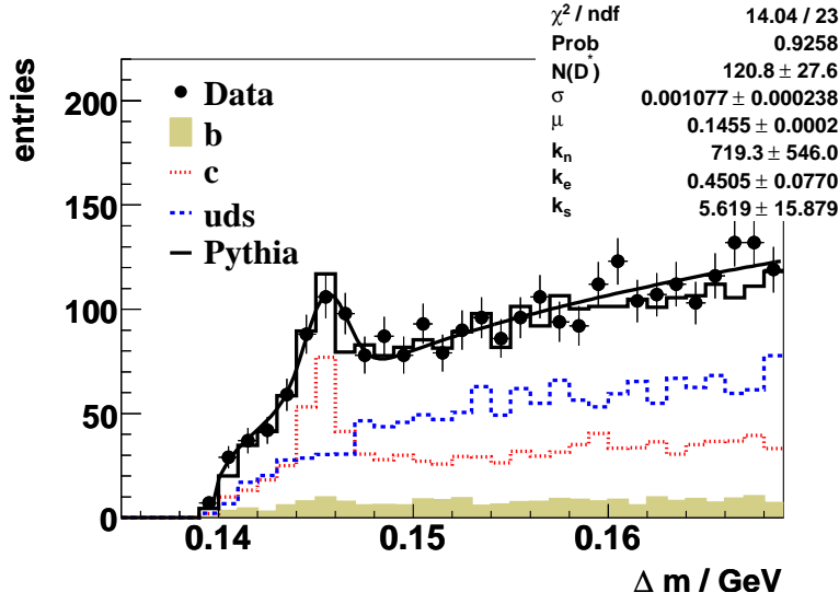
Figure B.1: Distribution of the mass difference of the D^* an D^0 candidates \Delta m = m_{K\pi\pi_S} - m_{K\pi} . The number of D^* events in the untagged photoproduction dijet sample determined by the fit is N^{D^*} = 121 \pm 28 .
