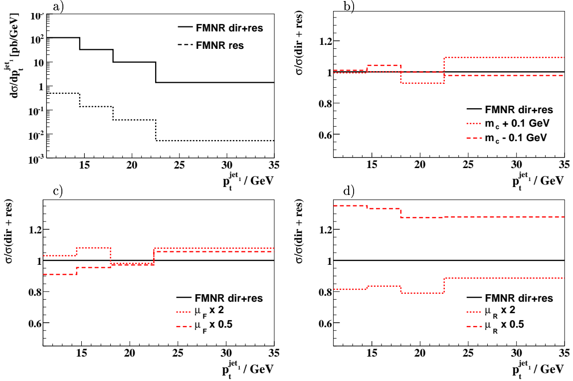
Figure 2.10: Results of the NLO calculations using the FMNR program for charm quarks as a function of p_t^{\text{jet}1} . a) Differential charm dijet cross section and the relative effect of varying b) the charm quark mass m_c , c) the factorisation scale \mu_F and d) the renormalisation scale \mu_R .
