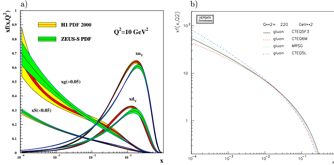
Figure 2.4: a) Gluon and valence quark ( u and d ) density of the proton as obtained from recent H1 and ZEUS fits. b) Gluon density of the proton as given by the CTEQ5F3 , CTEQ6M , CTEQ5L and MRST pdfs. The scale relevant in this analysis is given by \hat{p}_t^2 + m_Q^2 = 220 \text{ GeV}^2 .
