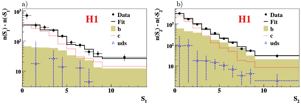
Figure 6.5: Distributions of a) the subtracted signed significance for the sample with exactly one selected track and b) the subtracted signed significance for the sample with two or more selected tracks. Only tracks with an impact parameter |\delta| < 0.1 cm are considered. The expectation from the PYTHIA Monte Carlo simulation is included in the figure, showing the contributions from the various quark flavours after applying the scale factors P_b = 1.98 , P_c = 1.45 and P_l = 1.44 as obtained from the fit.
