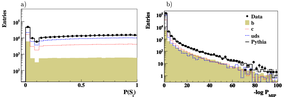
Figure 6.6: Distributions of a) the track probability P(S_i) and b) the negative logarithm of the multi impact parameter probability -\log(P_{MIP}) for both jets. Only tracks with an impact parameter |\delta| < 0.1 cm are used. The expectation from the PYTHIA Monte Carlo simulation is included in the figure, showing the contributions from the various quark flavours after applying the scale factors as obtained from the fit to the subtracted significance distributions.
