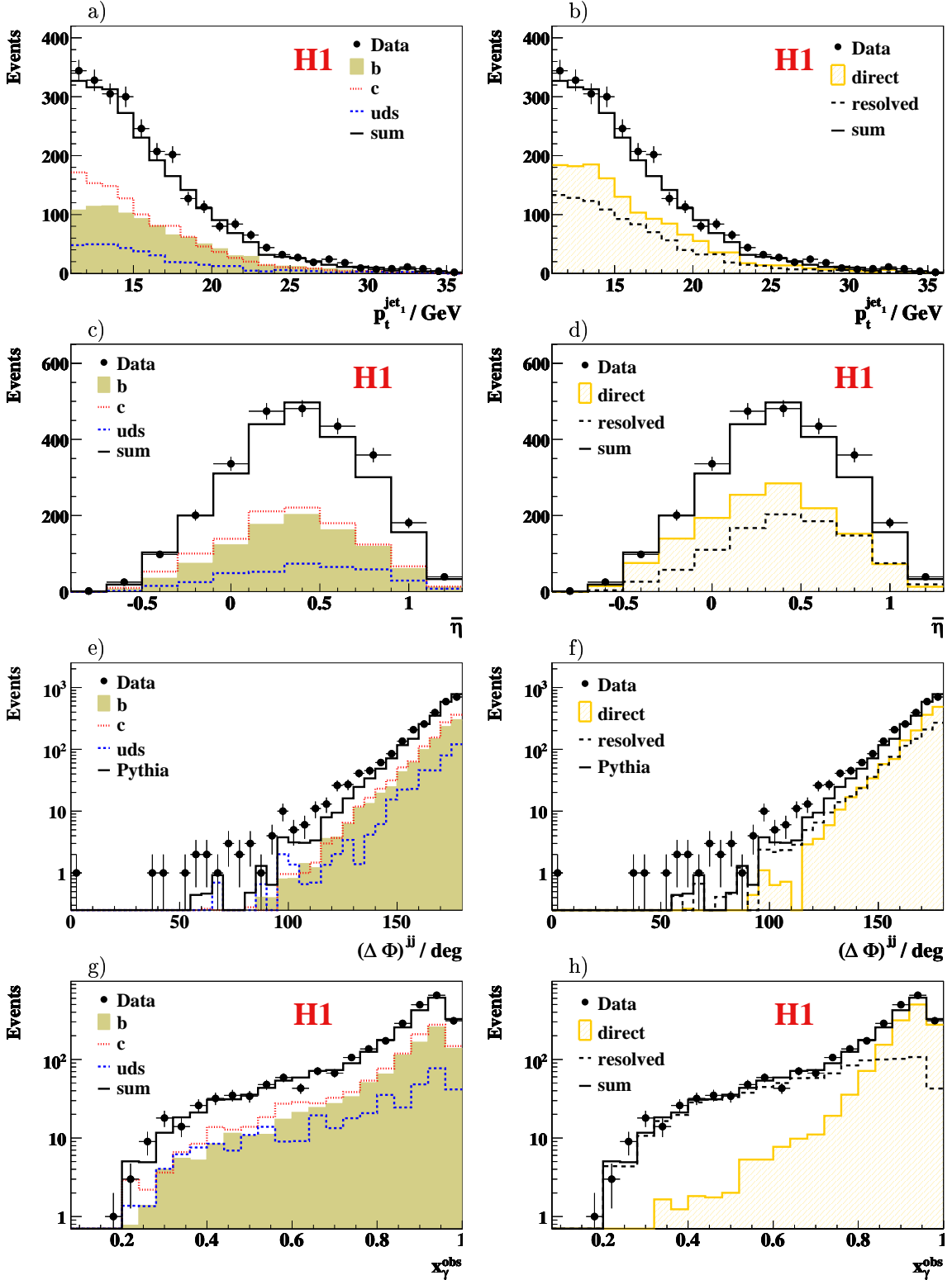
Figure 6.10: Distributions of the heavy quark enriched sample with two or more tracks originating from a secondary vertex and a decay length significance larger than 2.0. The left column shows the decomposition of the distribution into beauty, charm and light quarks after scaling the PYTHIA predictions by the scale factors obtained from the fit to the subtracted significance distributions of the full sample. In the right column the contributions from direct and resolved processes in PYTHIA are indicated as shaded histogram and dashed line respectively.
