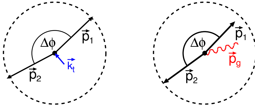
Figure 4.12: Two heavy quarks in the r\phi -transverse plane. An initial transverse momentum k_t \neq 0 of the incoming partons in the hard scattering (left) or gluon radiation (right) can lead to a non back-to-back topology of the outgoing partons. The picture is taken from [42].
