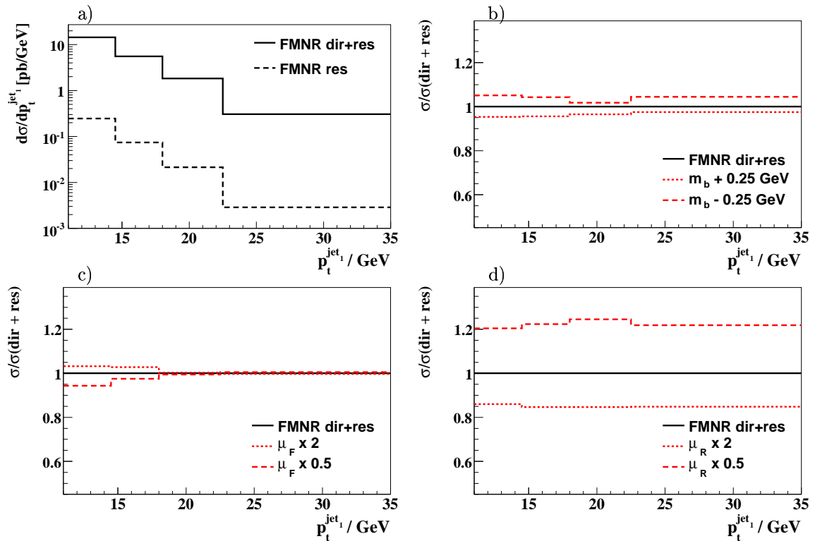
Figure 2.11: Results of the NLO calculations using the FMNR program for beauty quarks as a function of p_t^{jet1} . a) Differential beauty dijet cross section and the relative effect of varying b) the beauty quark mass m_b , c) the factorisation scale \mu_F and d) the renormalisation scale \mu_R .
