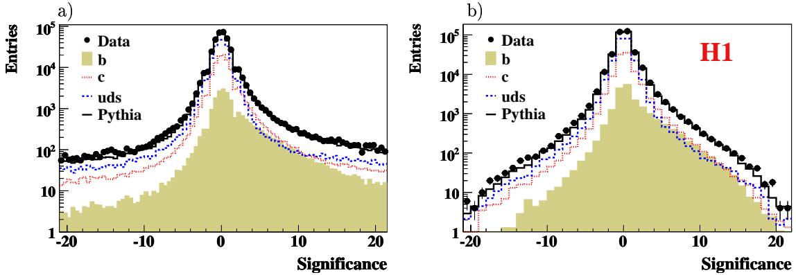
Figure 6.3: Distributions of a) the impact parameter significance for tracks and b) the impact parameter significance for tracks with |\delta| < 0.1 cm. The expectation from the PYTHIA Monte Carlo simulation is included in the figure, showing the contributions from the various quark flavours after applying the scale factors obtained from the fit to the subtracted significance distributions of the data (see section 6.3).
