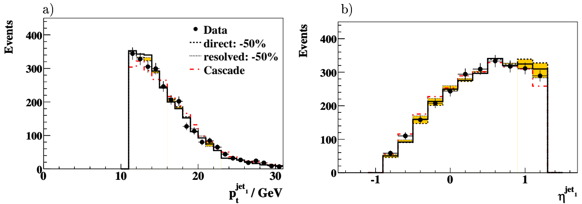
Figure 7.4: Distributions of p_t^{jet_1} and \eta^{jet_1} for the heavy flavour enriched sample (see section 6.6). The Monte Carlo distributions are normalised to match the data. Variations of the relative fractions of direct and resolved processes lead to the uncertainty band (shaded region). Cascade (dashed-dotted line) is shown separately.
