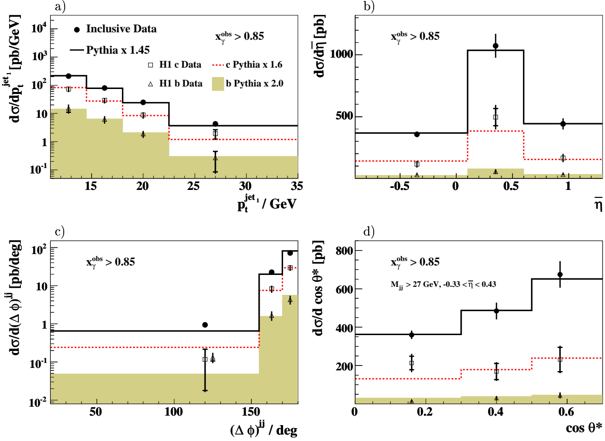
Figure 7.12: Differential flavour inclusive photoproduction cross sections a) d\sigma/dp_t^{jet1} , b) d\sigma/d\bar{\eta} , c) d\sigma/d(\Delta\phi)^{jj} and d) d\sigma/d\cos\theta^* for the process ep \rightarrow eq\bar{q}X \rightarrow ejjX in the region x_\gamma^{obs} > 0.85 . The inner error bars indicate the statistical uncertainty and the outer error bars show the statistical and systematic errors added in quadrature. The solid lines indicate the absolute prediction from PYTHIA scaled with a factor 1.45. The charm (boxes) and beauty (triangles) data are also shown together with the charm and beauty PYTHIA prediction scaled with the factors P_c(x_\gamma^{obs} > 0.85) = 1.6 and P_b(x_\gamma^{obs} > 0.85) = 2.0 .
