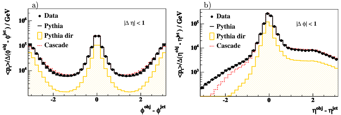
Figure 5.10: The transverse energy flow around the jet axis as a function of the distance to the jet axis in azimuthal angles \phi^{obj} - \phi^{jet} a) and as a function of the distance in pseudo-rapidity \eta^{obj} - \eta^{jet} (b).
