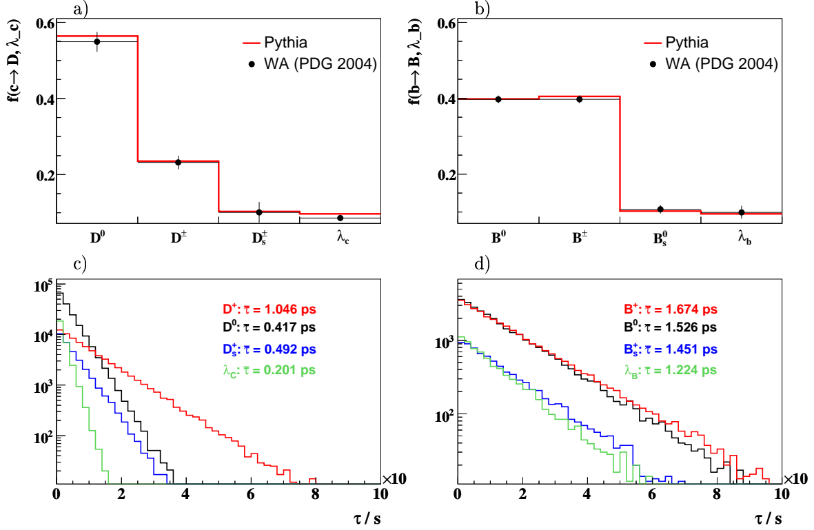
Figure 2.13: Branching ratios and lifetimes of charm and beauty hadrons. The properties have been calculated using the PYTHIA Monte Carlo simulation.
