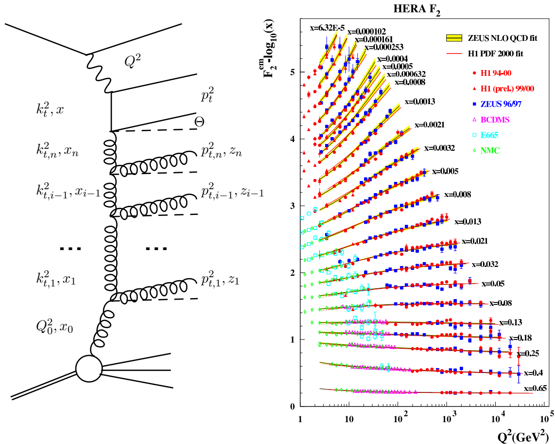
Figure 2.3: Parton evolution diagram (left). Measurement of the proton structure function F_2(x, Q^2) as a function of Q^2 at fixed values of x (right). Shown are the results from H1, ZEUS and various fixed target experiments. The lines correspond to the QCD fits performed by H1 and ZEUS.
