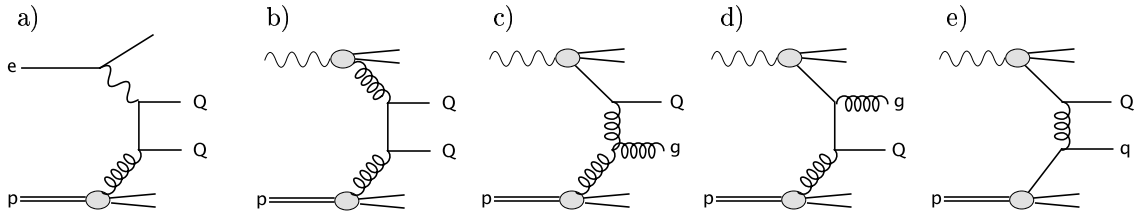
Figure 2.8: Heavy quark production processes in LO QCD: a) direct process (BGF) and b)-e) resolved processes. Heavy flavour excitation is shown in figures c)-e).
