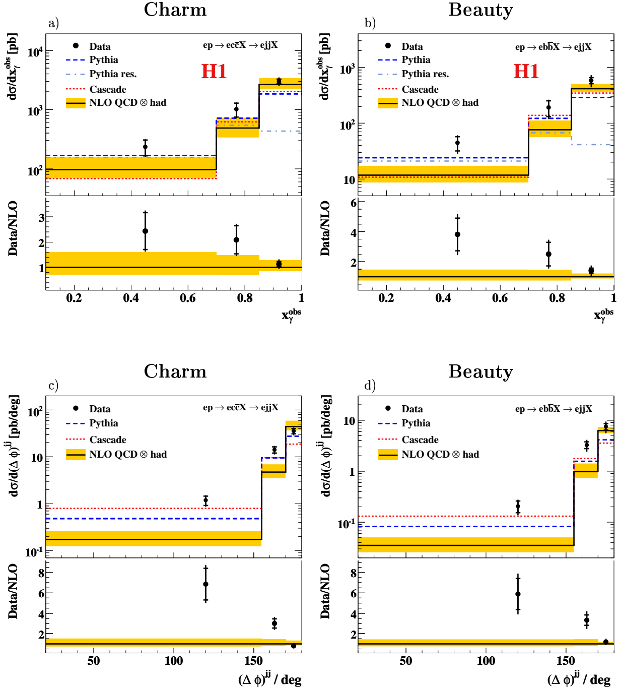
Figure 7.7: Differential charm and beauty photoproduction cross sections a, b) d\sigma/dx_\gamma^{obs} and c, d) d\sigma/d(\Delta\phi)^{jj} for the process ep \rightarrow e(c\bar{c} \text{ or } b\bar{b})X \rightarrow ejjX . The inner error bars indicate the statistical uncertainty and the outer error bars show the statistical and systematic errors added in quadrature. The solid lines indicate the prediction from a massive NLO QCD calculation, corrected for hadronisation effects, and the shaded band shows the estimated uncertainty. The absolute predictions from PYTHIA (dashed lines) and CASCADE (dotted lines) are also shown. The contribution from resolved processes in PYTHIA (dash-dotted lines) is depicted separately in figures a) and b).
