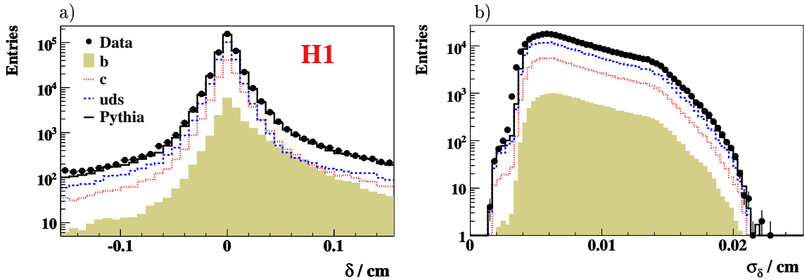
Figure 6.2: Distributions of a) the reconstructed impact parameter \delta and b) its error \sigma_\delta . The expectation from the PYTHIA Monte Carlo simulation is included in the figure, showing the contributions from the various quark flavours after applying the scale factors obtained from the fit to the subtracted significance distributions of the data (see section 6.3).
