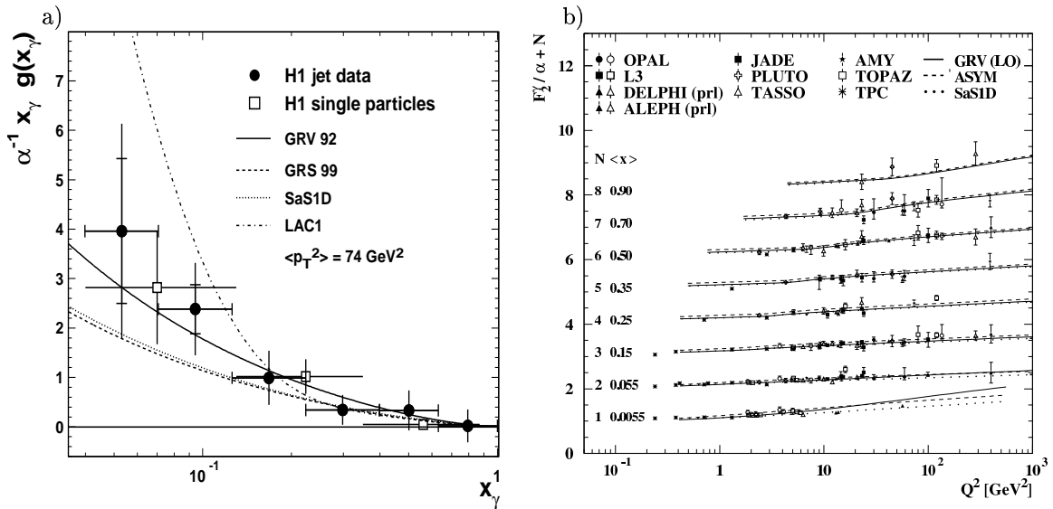
Figure 2.7: a) Measurement of the gluon distribution function of the photon from H1 [27] and b) summary of F_2^\gamma measurements from [26].
