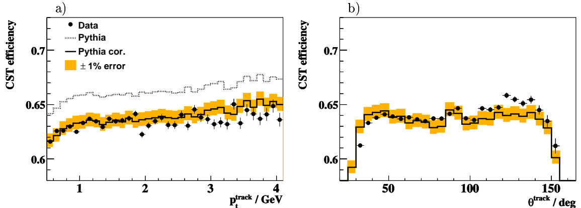
Figure 4.8: CST track finding efficiency for tracks with at least 2 CST hits and \mathcal{P}_{\text{Link}} > 0.1 as functions of p_t^{\text{track}} (a) and \theta^{\text{track}} (b). The Monte Carlo efficiency is shown separately for the default (dashed line) and modified (full line) version. The error band corresponds to a remaining uncertainty of \pm 1\% .
