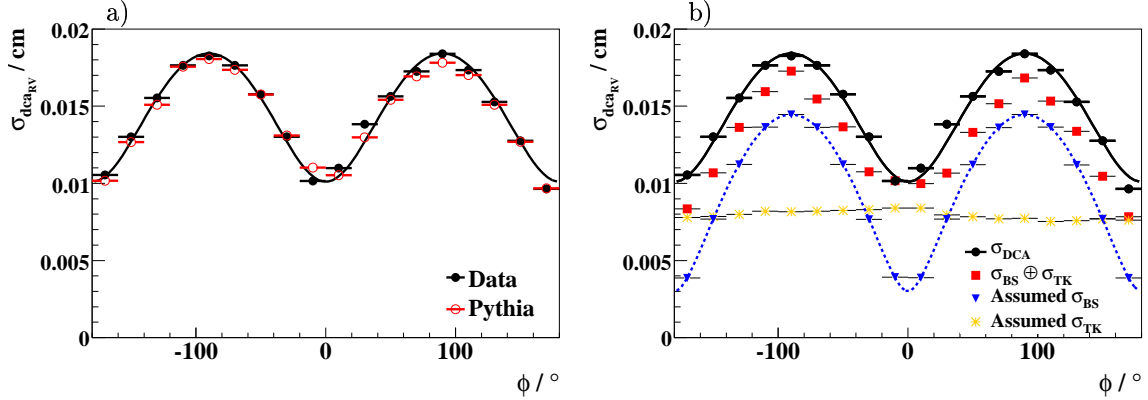
Figure 4.9: Gaussian width of the dca_{RV} distribution as a function of the track direction around the beam. Inclusive tracks with at least two CST hits and p_t > 0.5 \text{ GeV} are shown for data and simulation. The curves corresponds to a fit \sim \sigma_x^2 \sin^2(\phi) + \sigma_y^2 \cos^2(\phi) with the parameters \sigma_x = 145 \mu\text{m} and \sigma_y = 25 \mu\text{m} . On the right side the contributions from the beam spot \sigma_{BS} and the tracking resolution \sigma_{TK} are shown separately.
