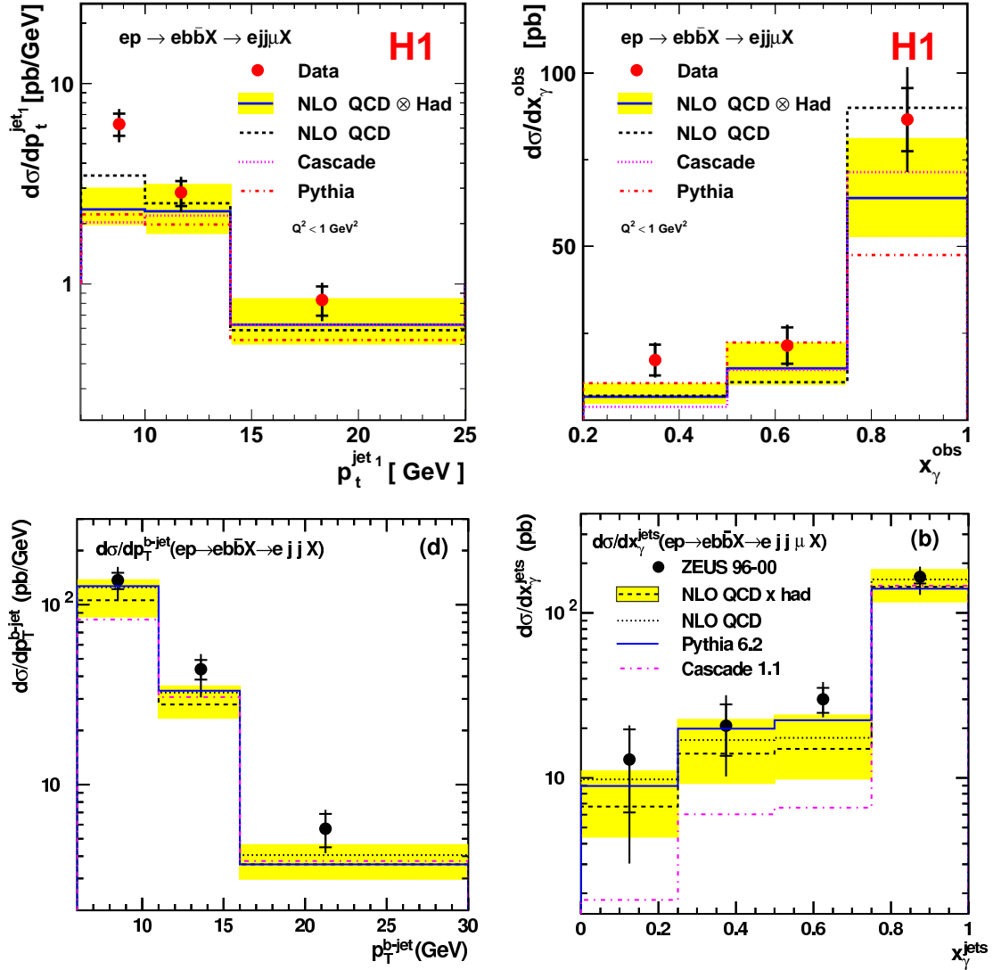
Figure 3.6: Differential beauty dijet photoproduction cross section as a function of p_t^{\text{jet}} and x_\gamma^{\text{obs}} from H1 [14] (top) and ZEUS [13] (bottom).
