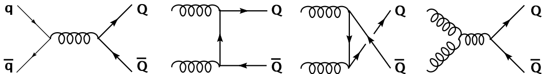
Figure 3.8: Leading order processes for charm and beauty quark production in p\bar{p} collisions.
