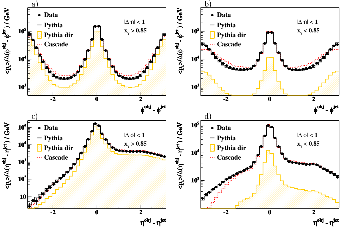
Figure 5.11: The transverse energy flow around the jet axis as a function of the distance to the jet axis in azimuthal angles \phi^{obj} - \phi^{jet} (a-b) and as a function of the distance in pseudo-rapidity \eta^{obj} - \eta^{jet} (c-d) for different x_\gamma^{obs} regions.
