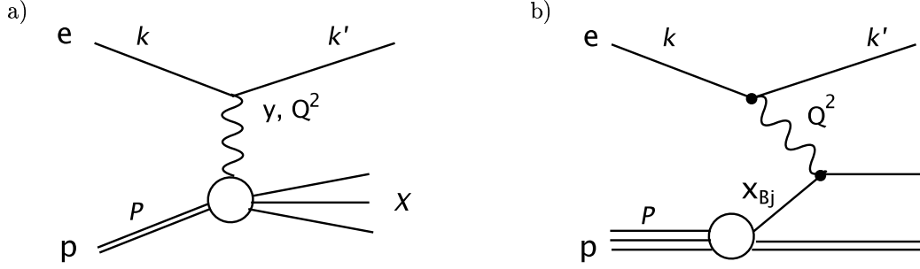
Figure 2.2: a) Electron-Proton scattering. b) Electron-Proton scattering in lowest order perturbation theory using the parton model.
