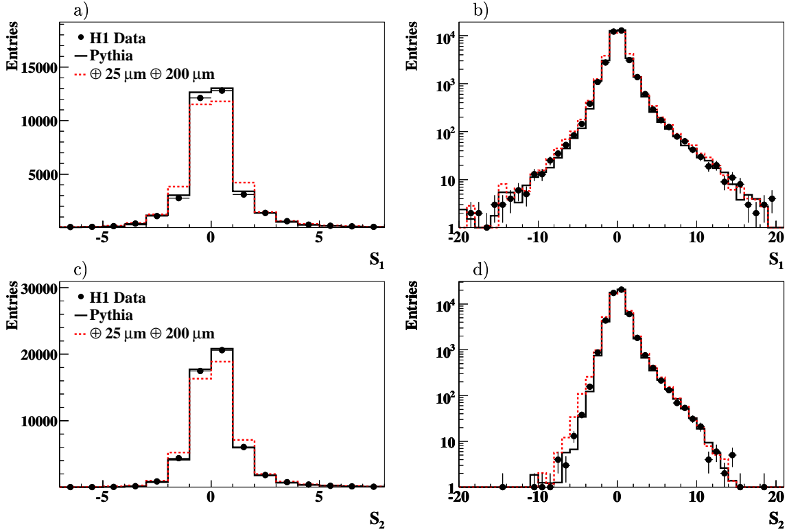
Figure 7.1: Distributions of the impact parameter significances S_1 and S_2 in linear (a and c) and semi-logarithmic scale (b and d). In addition to the default PYTHIA simulation (full line) a modified simulation is shown in which a Gaussian smearing of the impact parameter of 200 \mu\text{m} to 5% of randomly selected tracks and of 25 \mu\text{m} to the rest is applied (dashed line).
