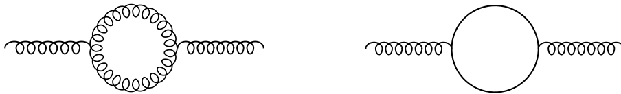
Figure 2.1: Higher order correction diagrams with gluons. Left: gluon loop. Right: fermion loop.
