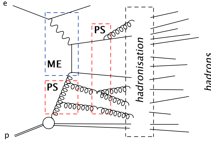
Figure 2.12: Schematic view of the subsequent steps of an event generator: matrix element (ME), parton shower (PS) and hadronisation.
