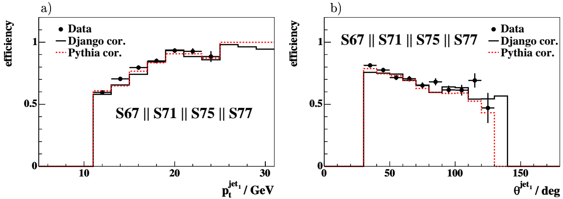
Figure 5.5: The trigger efficiency for the combination of all subtriggers as a function of the transverse momentum (a) and the polar angle (b) of the leading jet after correction.
