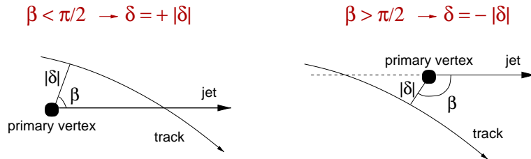
Figure 4.3: Sign convention of the impact parameter \delta .
