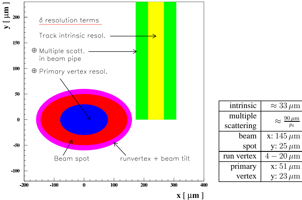
Figure 4.6: Schematic view of the various contributions to the impact parameter resolution taken from [74]. The numbers in the table correspond to the 1999-2000 data taking phase.
