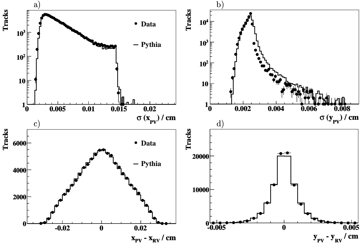
Figure 4.5: The calculated errors on the primary vertex positions (top) and the difference of the reconstructed primary vertex and the run vertex (bottom). H1 data are shown and compared with the PYTHIA simulation.
