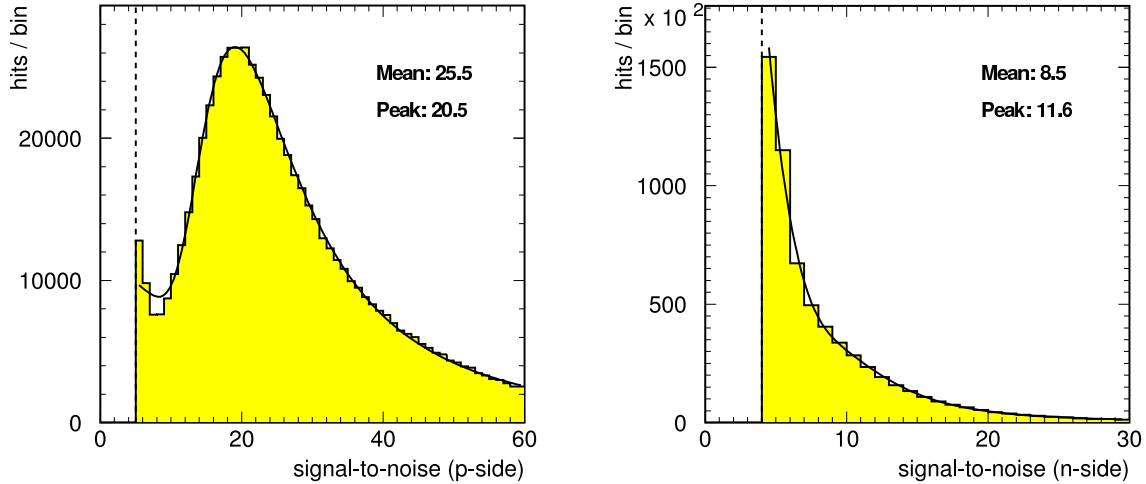
Figure 3.4: Signal-to-noise ratio for the p -side (left) and n -side (right). The dashed line marks the cut made in the hit finding algorithm.
