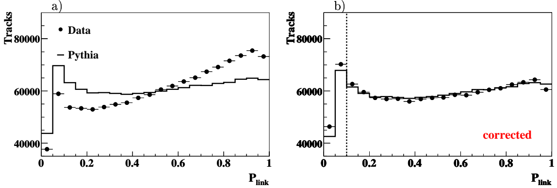
Figure 4.7: Distribution of the CJC-CST link probability \mathcal{P}_{Link} before (left) and after correction (right). The vertical dashed line indicates the cut applied in the track selection. See text for details.
