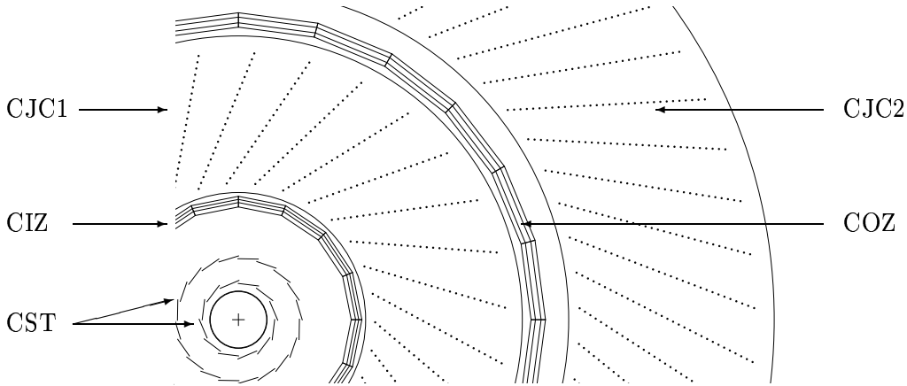
Figure 3.2: Radial view of the central tracking system (section).
