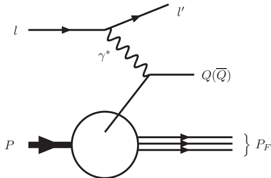
Figure 5: LO intrinsic heavy quark production.
