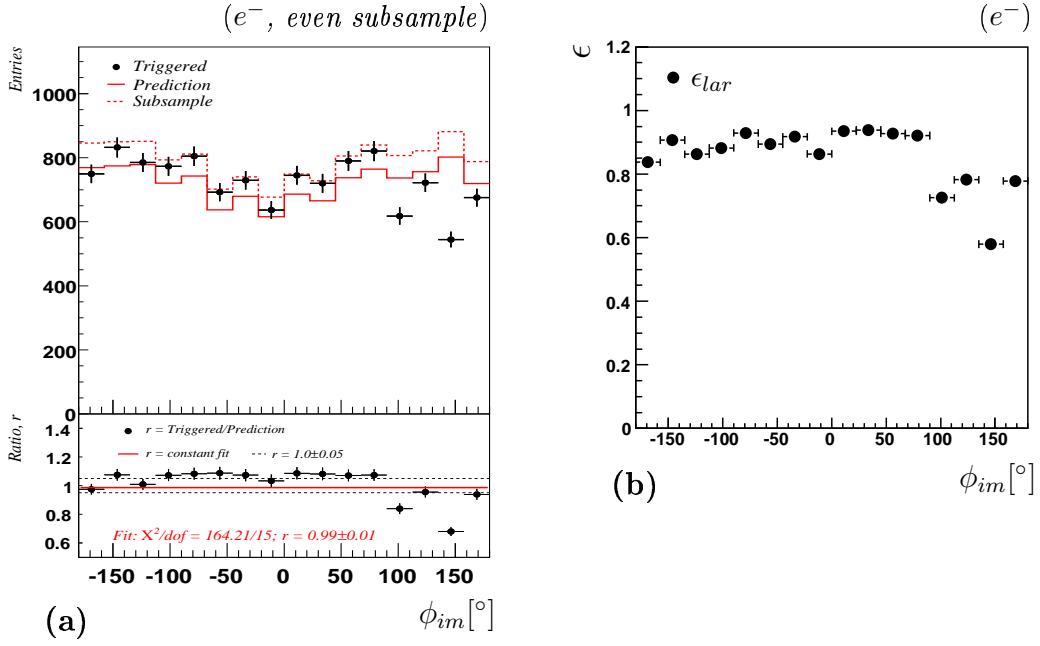
Figure 7.17: (a) The \phi -impact \phi_{im} distribution for the even subsample, LAR triggered events and the prediction. The ratio r = n_e/n'_e between the number of triggered events and the prediction together with a y = \text{constant} fit are shown. The E'_e - z_{im} binning used for the odd efficiency corresponds to that used in the analysis. (b) \epsilon_{lar} as a function of \phi_{im} .
