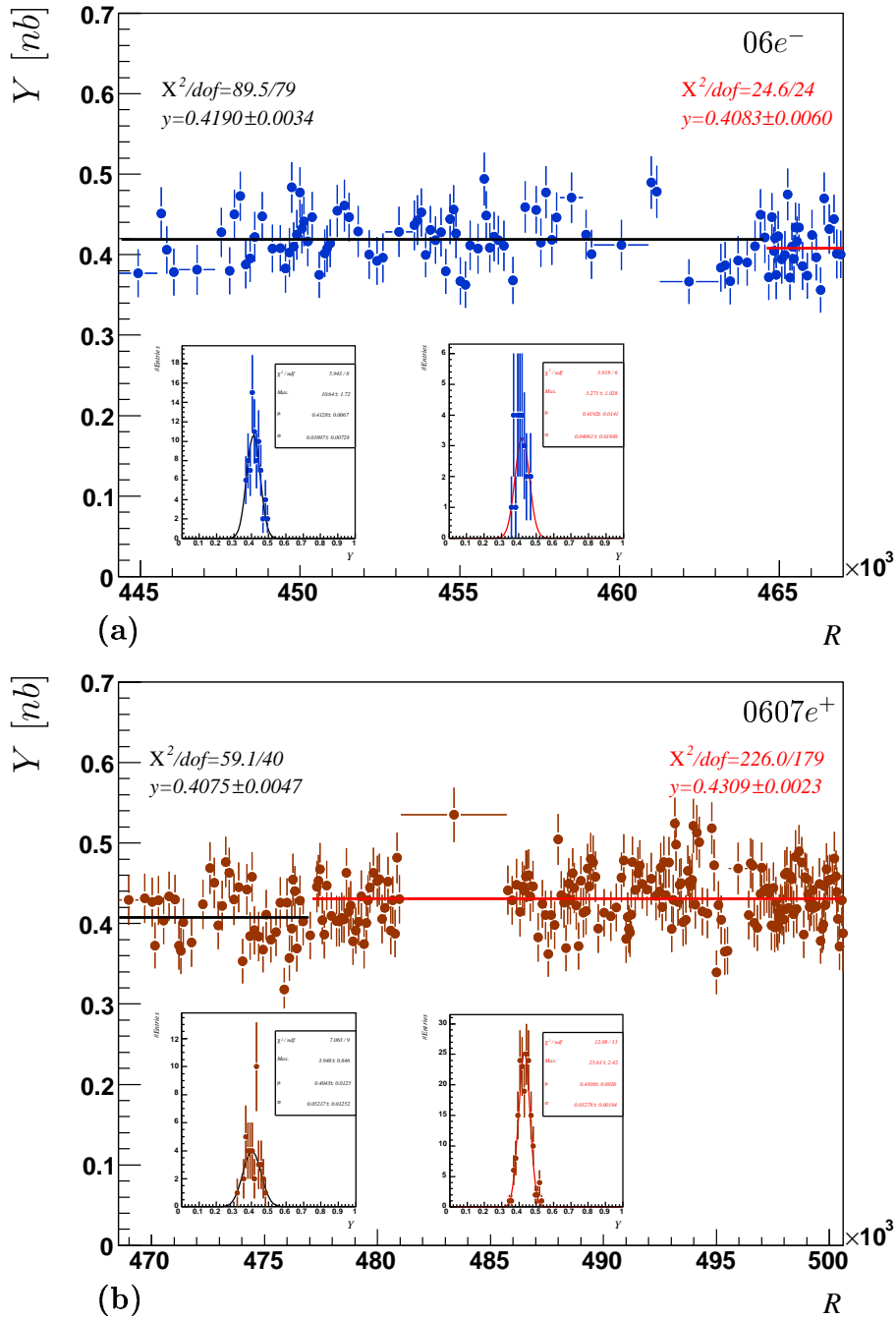
Figure 7.39: (a) The event yield Y for the 06e^- period as a function of the run number R . Fitted to the data are two functions of the form Y = \text{constant} over the indicated run ranges. The inner plots show the result of a Gaussian fit to the two yield distributions corresponding to the fitted runranges. (b) Similar plots for 0607e^+ period.
