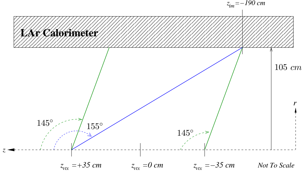
Figure 6.15: Schematic showing the dependence of the electron polar angle acceptance on the z -coordinate of the reconstructed vertex.
