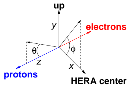
Figure 3.6: The ZEUS reference coordinate system.
