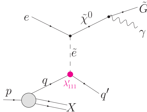
Figure 7.1: Feynman diagram for the signal process. The neutralino decays dominantly into a photon \gamma and a gravitino \tilde{G} .
