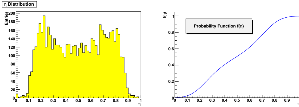
Figure 5.5: Example \eta and corresponding f distribution.
