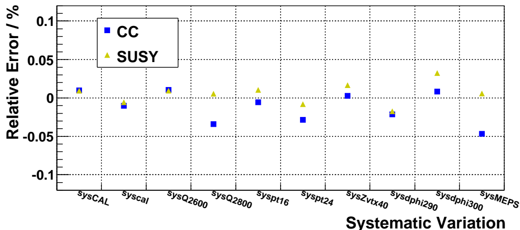
Figure 10.1: Sources of Systematic Uncertainties. sysCAL ( syscal ) denotes the greatest positive (negative) energy scale uncertainty, sysQ2600 ( sysQ2800 ) the change of the Q^2 cut 100 \text{ GeV}^2 down (up), syspt16 ( syspt24 ) the change of the missing p_T cut 4 \text{ GeV} down (up), sysZvtx40 the 10 \text{ cm} relaxing of the Z -vertex cut, sysdphi290 ( sysdphi300 ) the change of the \Delta\phi(\gamma, \text{jet}) cut 50 \text{ mrad} down (up), and sysMEPS denotes the change of the QCD radiation model to MEPS.
