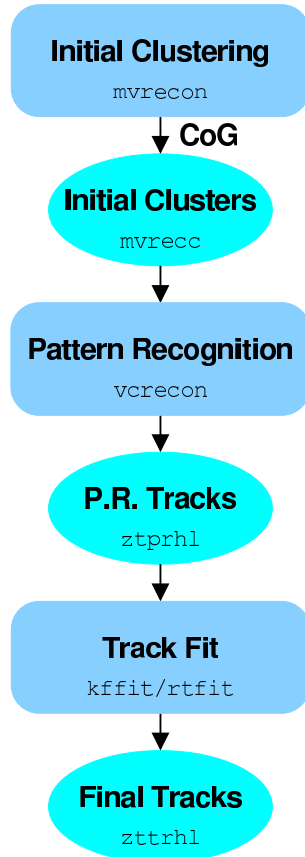
Figure 5.2: Tracking Chain
