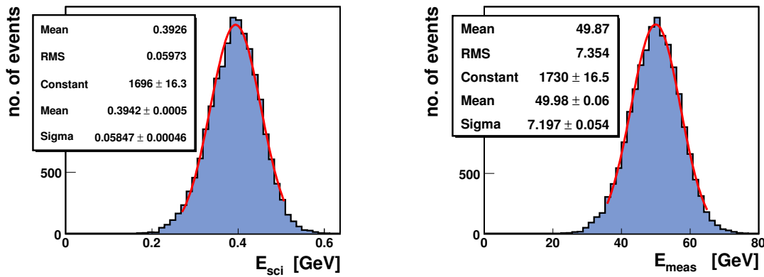
Figure 4.5: Illustration of the calibration of the simulated CMS HCAL with 50 GeV pions. Left: scintillator signal before calibration. Right: simulated measured energy, consisting of the scintillator signal times a calibration factor “C” plus a small contribution of energy depositions from the ECAL. The red line represents a Gaussian fit to the distribution.
