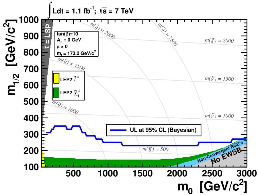
Figure 8.2: Exclusion line ( blue ) in the m_0 - m_{1/2} -plane of the cMSSM. The line corresponds to an Upper Limit (UL) for the exclusion at a 95% Credibility Level (CL) in Bayesian statistics. The area below the blue line is excluded. The yellow and green bands indicate regions excluded by LEP 2. For the right lower corner no reasonable solution exists within the cMSSM. The gray lines mark constant gluino ( \tilde{g} ) and squark ( \tilde{q} ) masses.
