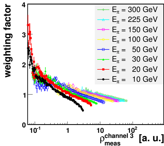
Figure 4.2: WFs for the third channel of the readout scheme “1-4-4-8” as a function of the energy density \rho_{\text{meas}}^i . The color code refers to the energy E_{\pi} of the simulated incident pions.
