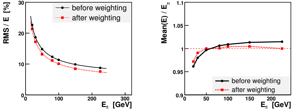
Figure 4.11: Energy resolution (left) and linearity (right) before (solid black) and after weighting (red dashed) for the “1-4-4-8” readout design. As a consistency check the entry at 80 GeV has been added. For this energy no WFs exist. The errors are so small that they lay within the markers.
