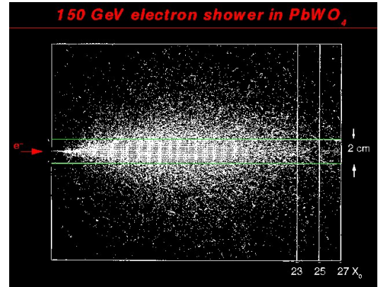
Figure 3.6: Simulation of an electromagnetic shower in lead tungstate, caused by an electron with an energy of 150 GeV. Green lines illustrate the size of a crystal in the ECAL of CMS. From [65].
