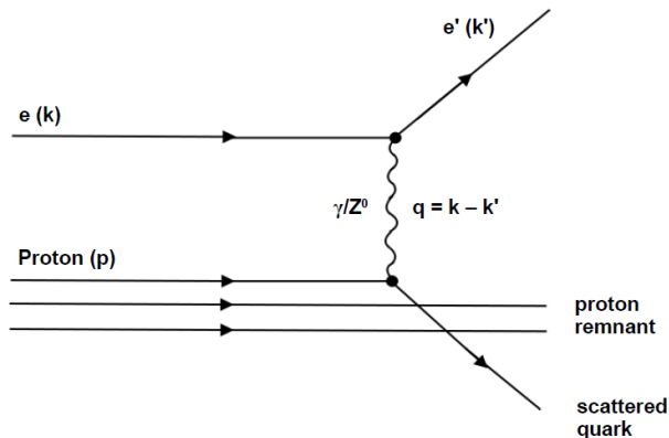
Figure 1.2: Schematic representation of lepton-proton scattering.
