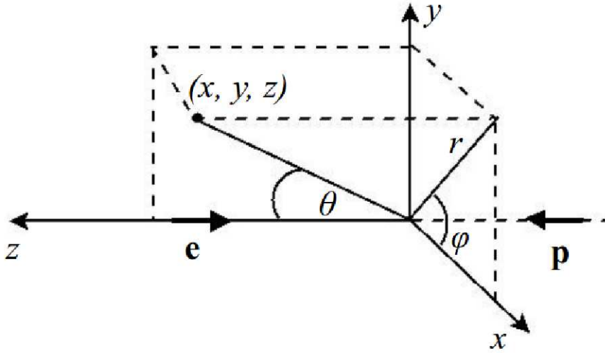
Figure 2.3: The coordinate system at H1
