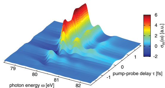
FIG. 3. (Color online) Attosecond XUV transient absorption spectrum \sigma_m(\omega; \tau) [see Eq. (14)] of krypton as a function of energy \omega and pump-probe delay \tau .
