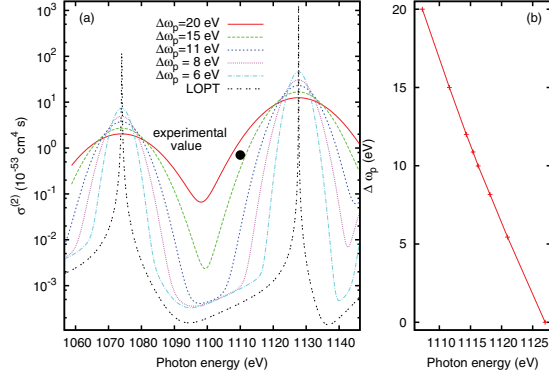
FIG. 3. (Color online) (a) Two-photon ionization cross section for \text{Ne}^{8+} , given by Eq. (8). The perturbative result \sigma_{\text{LOPT}}^{(2)} of Eq. (9) (dotted line) is taken as a reference signal for averaging over different bandwidths (FWHM) of the pulses. The point at 1110 eV corresponds to the experimental value of 7 \times 10^{-54} \text{ cm}^4 \text{ s} reported in Ref. [6]. (b) Relation between the bandwidth \Delta\omega_p and the mean photon energy \omega_{\text{in}} for which the two-photon ionization cross section \sigma_{\text{incoh}}^{(2)} is fixed at 7 \times 10^{-54} \text{ cm}^4 \text{ s} .
