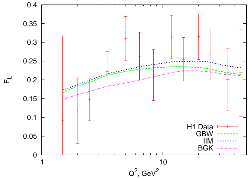
Figure 49: The proton structure function F_L as a function of Q^2 . The data are given in [84]. The full error bars indicate the total uncertainty. The dashed lines show the predictions of F_L obtained from the different dipole model fits to data used in this analysis.
