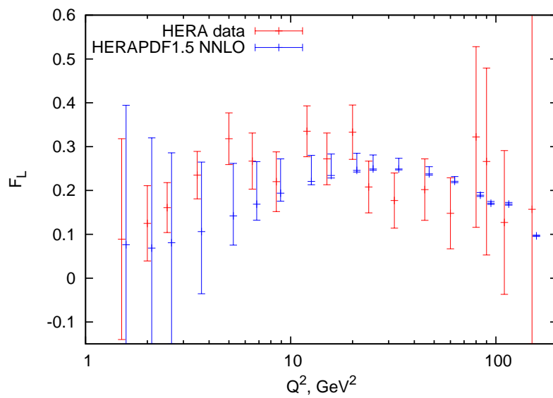
Figure 61: The obtained averaged values of the longitudinal structure function F_L together with the prediction from NNLO HERAPDF1.5 [48]. The error bars represent total uncertainties.
