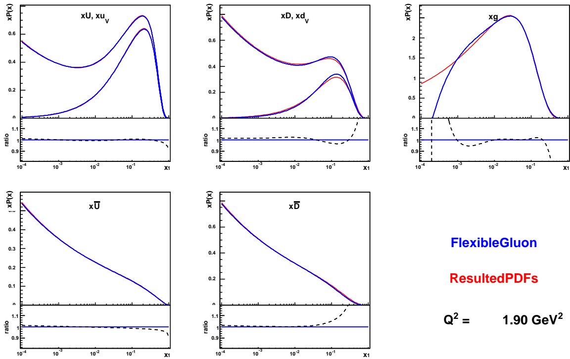
Figure 36: The PDFs extracted from the NLO DGLAP fit to the combined HERA I and combined reduced proton beam energy E_p = 460, 575 GeV data at the starting scale Q^2 = 1.9 GeV 2 . The red curve shows the PDFs obtained using the resulted parametrization. The blue curve in turn shows the PDFs extracted using the flexible gluon parametrization (72). The gluon distribution becomes negative at low x . The bottom panel shows the ratios of the extracted PDFs using the resulted parametrization to the PDFs obtained with the flexible gluon parametrization.
