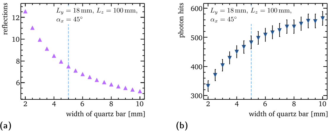
Figure 5.4: Influence of the channel width on (a) the number of reflections a photon undergoes before detection and (b) the measurable light. The dashed blue lines indicate the width used for the prototype detector described in chapter 6.
