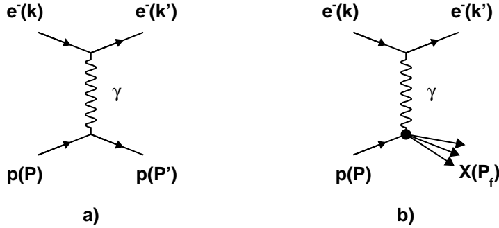
Figure 2.1: Scattering of electron on point-like proton a). Scattering of electron on realistic proton b).
