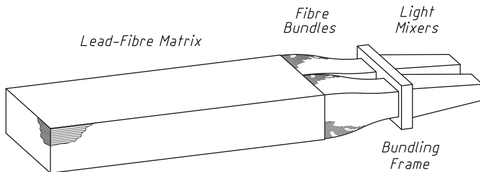
Figure 3.5: Sketch of a single SPACAL module.
